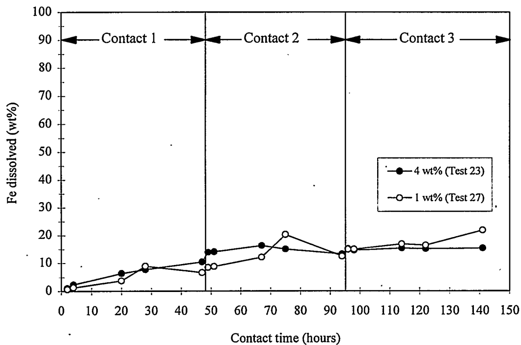
Figure 3.13 Percent Fe Dissolved in Cs-Elution Tests Using 4 and 1 wt% Oxalic Acid in the Presence of Additional \text{Fe}_2\text{O}_3
