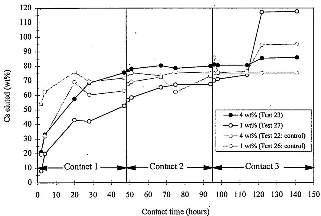
Figure 3.11. Percent Cs Eluted from Zeolite During Multiple-Contact Tests Using 4 and 1 wt% Oxalic Acid in the Presence of Additional \text{Fe}_2\text{O}_3
