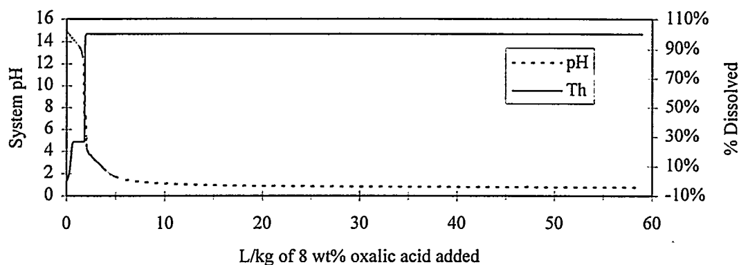
Figure O.12(a). Percent of Modeled Sludge Th Dissolved at Thermodynamic Equilibrium for 0 - 60 L 8 wt% Oxalic Acid/kg Sludge
