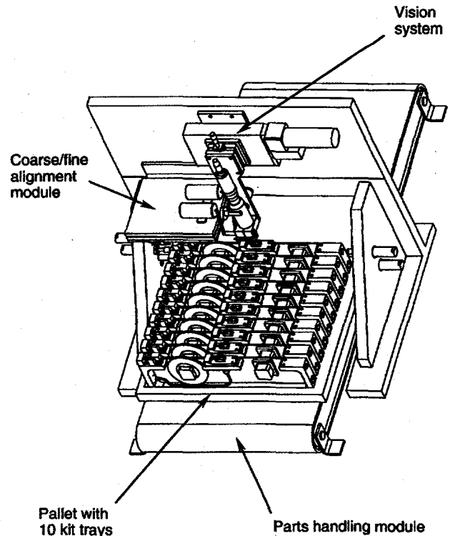
Figure 1. The Ortel AFPM has one high-precision stage mounted on the left side of the frame.
