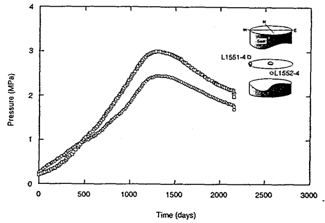
Figure 11. Internal pressure data for 100% bentonite core seal.
