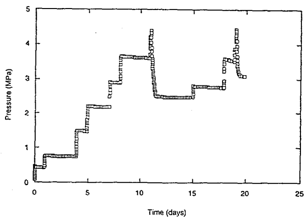
Figure 3. Results of gas flow testing of a 100% bentonite core seal.
