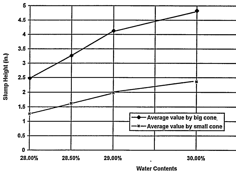
Figure 3.25 Curve of Slump test results
