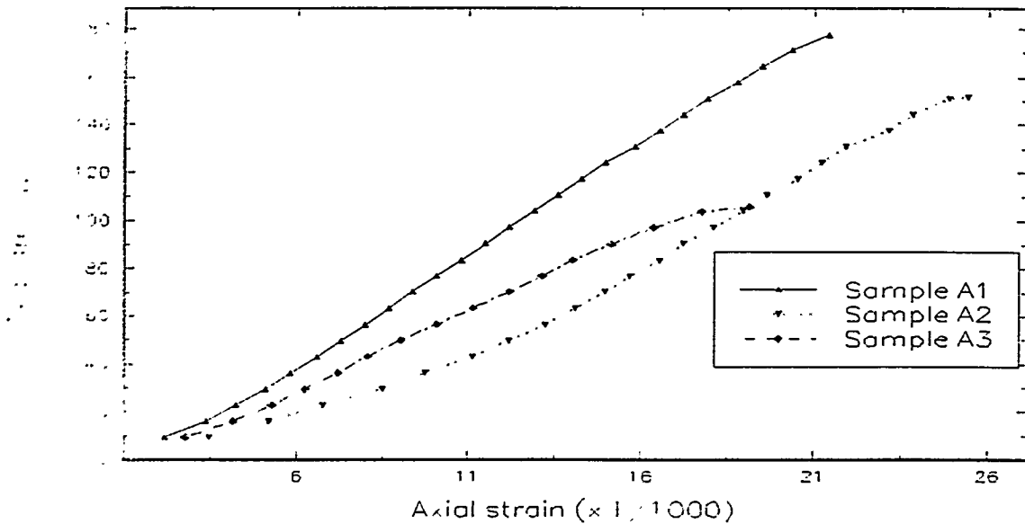
Figure 3.17 Stress-strain relationship curve of sample group 3 (40% F.A., 55% S.S, 5% L.W., mixed with 29% water)
