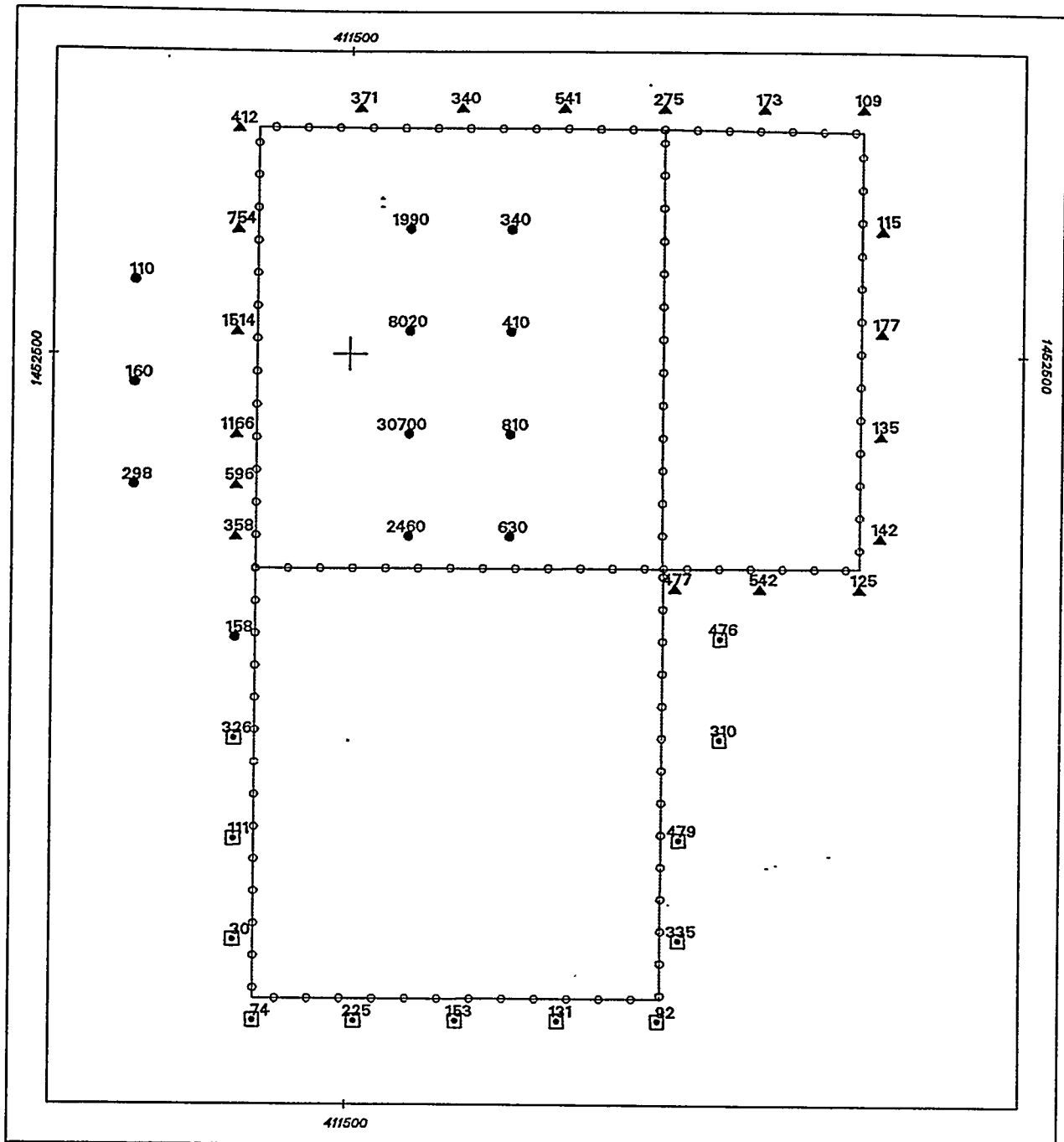
Figure 5-1 Total VOCs (ppbv) in Soil Gas at 10ft, Mixed Waste Landfill
