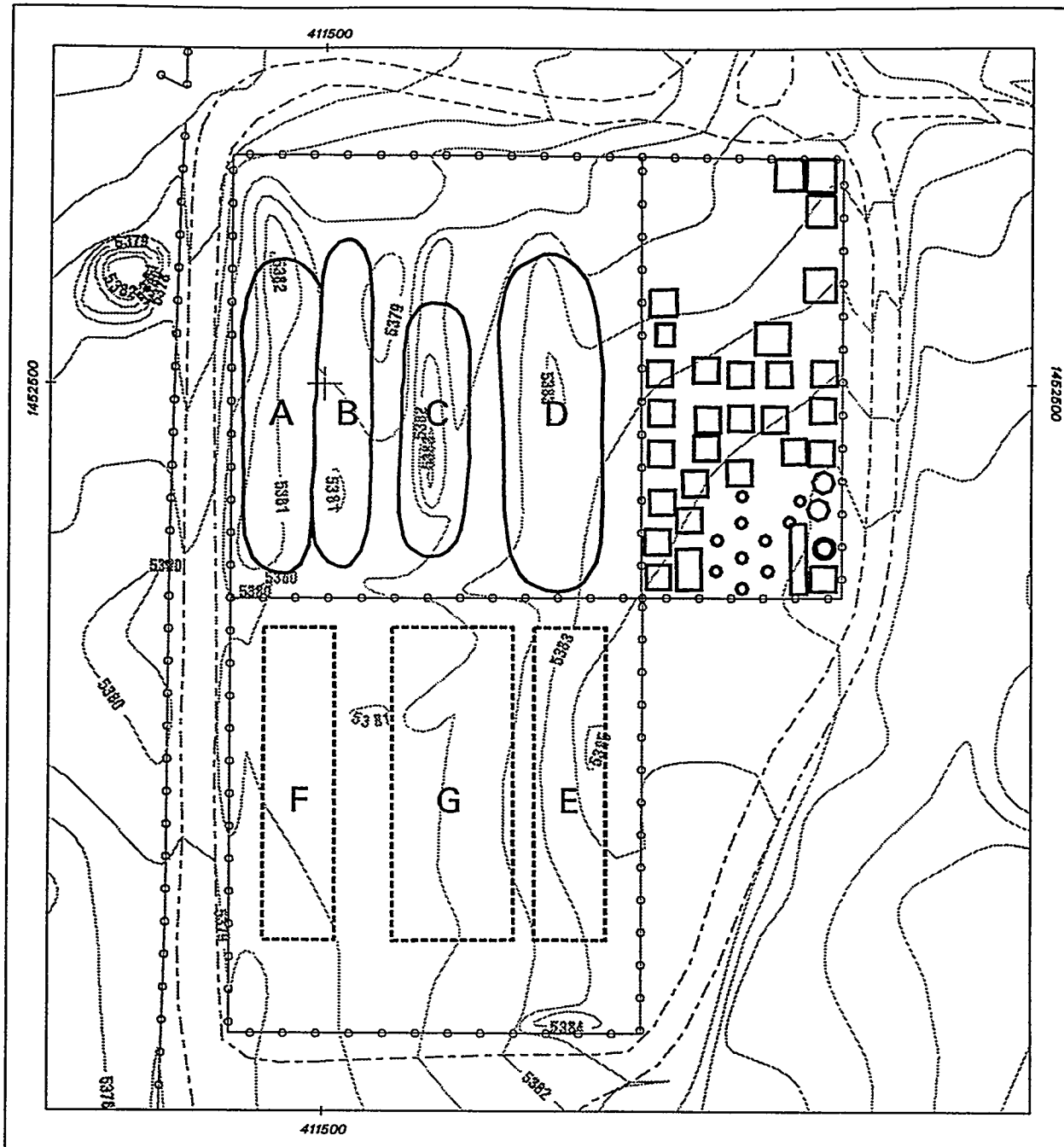
Figure 1-3 Mixed Waste Landfill
