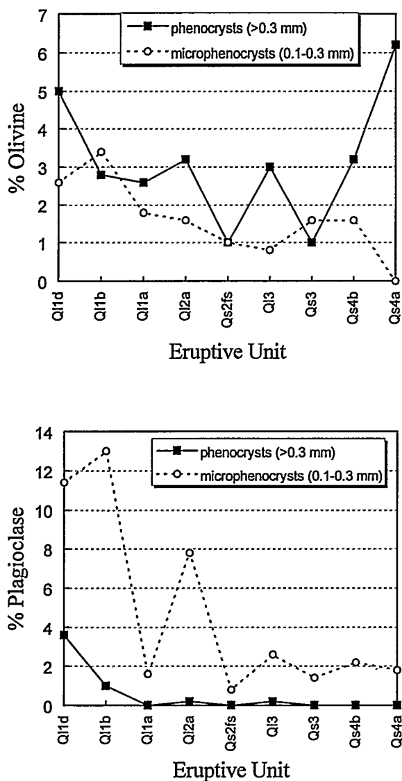
Figure 8. Percent olivine and plagioclase phenocrysts and microphenocrysts determined by point counting for representative samples of eruptive units from the Lathrop Wells volcanic center. Samples counted from each eruptive unit are LW20FVP from Ql1d, LW73FVP from Ql1b, LW11FVP from Ql1a, LW40FVP from Ql2a, LW97FVP from Qs2fs, LW61FVP from Ql3, LW80FVP from Qs3, LW78FVP from Qs4b and LW151 from Qs4a.
