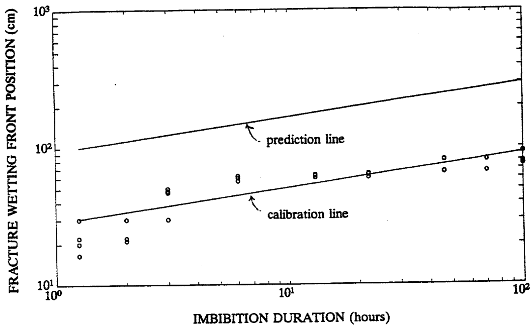
Figure 5.4: Fracture wetting front position; observed (circles) and calibrated (line).
