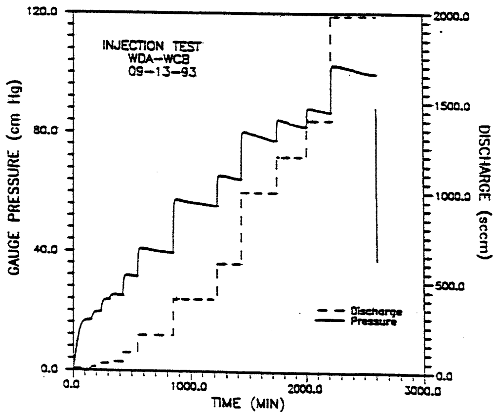
Figure 6.7: Pressure response during a multi-step injection test.
