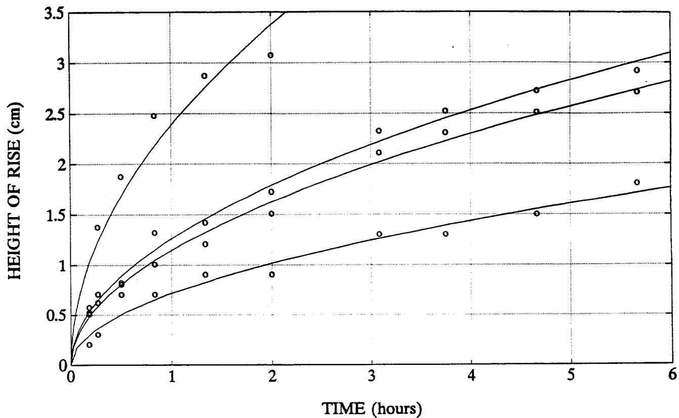
Figure 4.3: Height of water rise in rock matrix; observed (symbols) and calibrated (lines)
