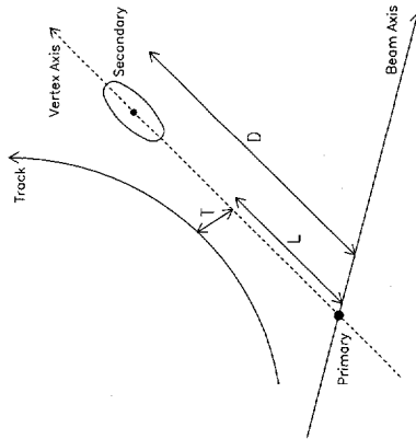
Figure 6: Impact parameter of a track to the vertex axis.
