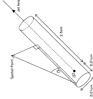
Figure 4: Construction of \alpha , the angular displacement.
