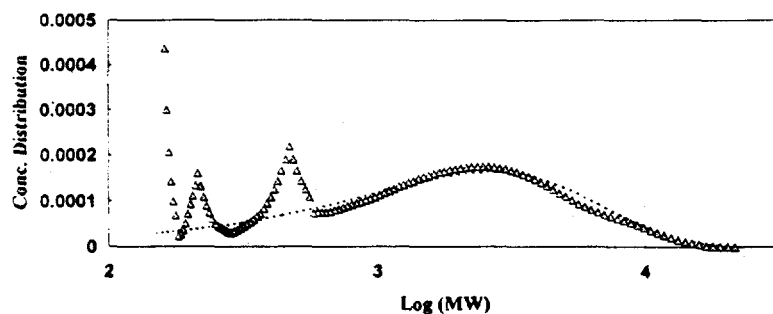
Figure 2. Comparison of experimental results of MWD with model simulation at 150 C, 25% tetralin and at a residence time of 42.51 minutes (Δ: experimental data; .....: Gamma Distribution fit).
