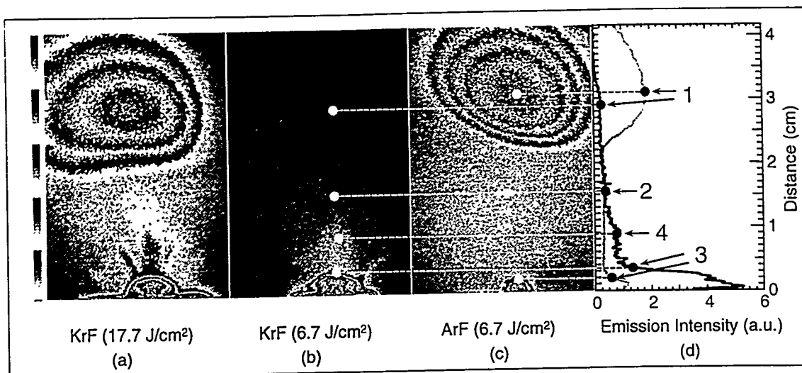
Fig.1. Gated-ICCD photographs of the total visible luminescence at \Delta t = 800\text{--}850 ns following ablation of pyrolytic graphite in vacuum using (a) KrF-laser ( 17.7\text{ J/cm}^2 ), (b) KrF-laser ( 6.7\text{ J/cm}^2 ) and (c) ArF-laser ( 6.7\text{ J/cm}^2 ) irradiation (incident angle 30^\circ from the left). The 5-grayscale palette (shown at the left) is normalized to the maximum numbers of counts for each image. (d) A line-profile of the emission intensity from the irradiated spot along the target normal shows the relative emission intensities of the different plasma components for (1) the fast, ball-shaped component of Fig.1(c) and the shell-shaped component in Fig.1(b); (2) the slower 'second' component of atomic emission; (3) the even slower 'third' component near the target surface and (4) the jets of \text{C}_2 which extend between the third and second components. The line profiles are normalized to the intensity of the 2nd-component.
