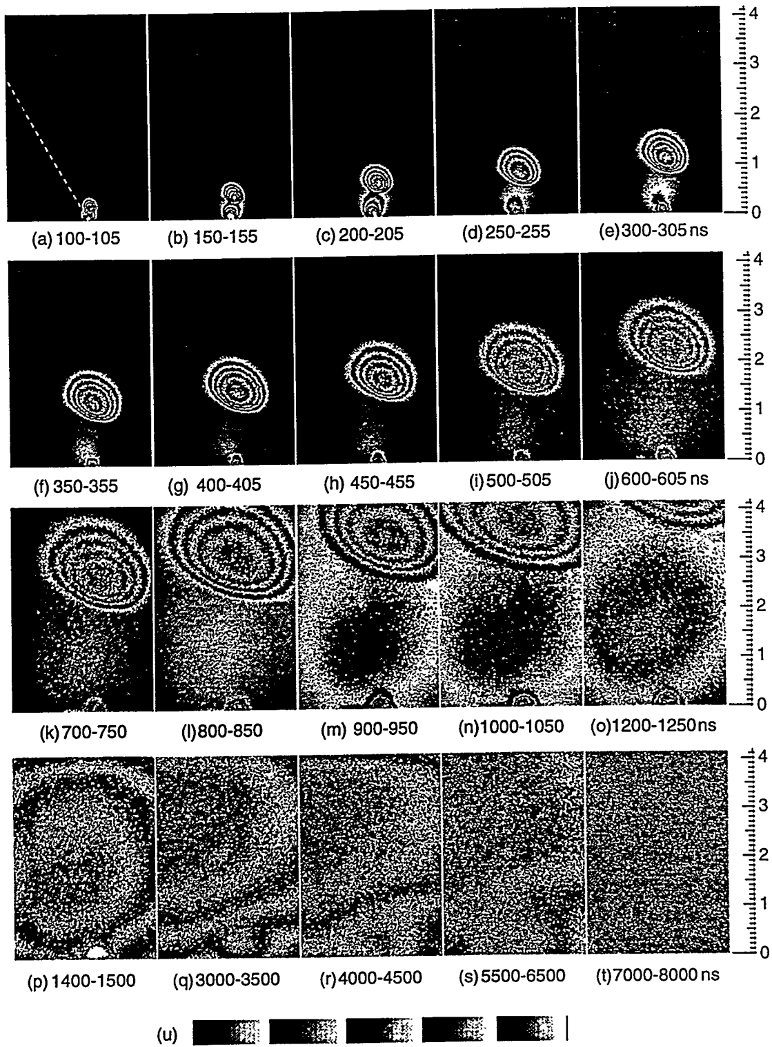
Fig.2. Gated-ICCD images of ArF-laser generated ( 6.7 \text{ J/cm}^2 ) plasmas taken at the indicated times [i.e. from (a) 100 ns delay, 5 ns-gate to (t) 7000 ns delay, 1000 ns-gate] following the laser pulse. (u) The 5-grayscale palette is normalized to the maximum emission intensity of the 1st-plasma component for images (a)-(o), and to the maximum of the 2nd component for (p)-(t). Figure 2(l) and Fig. 1(c) are the same. Laser incidence angle was 30^\circ [from the left, see dashed line in (a)].
