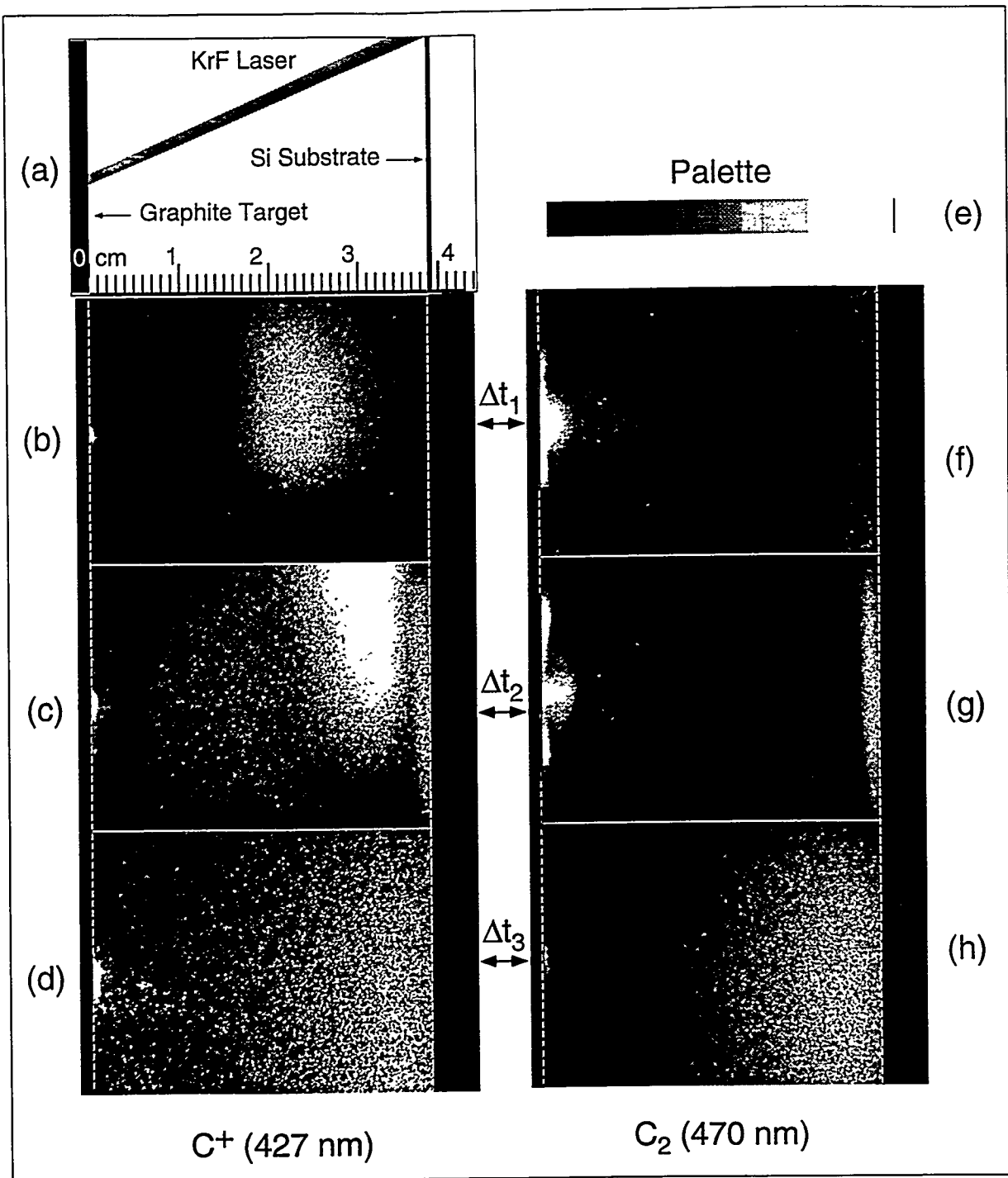
Fig.4. Species-resolved images of the KrF-laser ( 17 \text{ J/cm}^2 ) generated plasma luminescence between a graphite target and an unheated silicon substrate, as shown schematically in (a). Images (b)-(d) are taken through a 427 nm filter ( \text{C}^+ emission line) while images (f)-(h) on the right are taken through a 470 nm filter ( \text{C}_2 ( \Delta v = +1 ) Swan band). The pairs of images were acquired at the following times following the laser pulse: (b),(f) \Delta t_1 = 575\text{-}675 \text{ ns} ; (c),(g) \Delta t_2 = 775\text{-}975 \text{ ns} ; and (d),(h) \Delta t_3 = 10\text{-}12 \text{ }\mu\text{s} . (e) Grayscale palette used for representation of the intensities.
