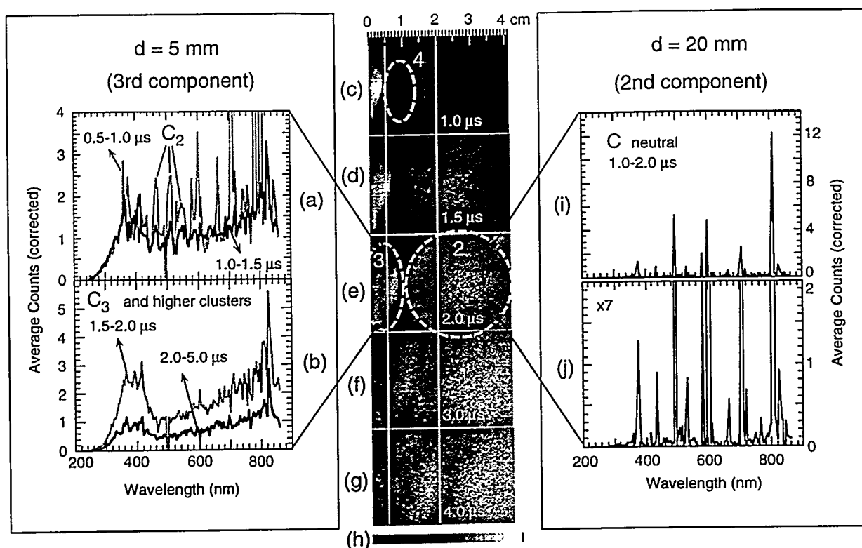
Fig. 5. Spectrally-corrected gated photon counting emission spectra of the carbon plume expansion into vacuum following KrF-laser ( 7 \text{ J/cm}^2 ) ablation of pyrolytic graphite. As shown in the unfiltered ICCD images (c)-(g), two distances were chosen for study [(a),(b) d = 5 \text{ mm} and (i),(j) d = 20 \text{ mm} ] in order to investigate the two regions of weak plasma luminescence demarcated in (e). Delays/exposures are (c) 1.0 \mu\text{s}/10 \text{ ns} , (d) 1.5 \mu\text{s}/50 \text{ ns} , (e) 2.0 \mu\text{s}/100 \text{ ns} , (f) 3.0 \mu\text{s}/200 \text{ ns} , (g) 5.0 \mu\text{s}/500 \text{ ns} . As shown in (c), the jets of emission present at d = 5 \text{ mm} until \Delta t = 1.0 \mu\text{s} are comprised of \text{C}_2 emission bands (see gray curve in (a) 0.5\text{--}1.0 \mu\text{s} ). The 3rd component emission spectrum is a broad continuum (see the three spectra in (a) and (b) for \Delta t > 1.0 \mu\text{s} ) as it propagates across the d = 5 \text{ mm} position (shown in (d)-(g)) with a distinguishable band of \text{C}_3 emission at 400 \text{ nm} . Spectra (i) and (j) represent the emission collected from the 2nd component at d = 20 \text{ mm} from 1.0\text{--}2.0 \mu\text{s} (as imaged in (c)-(e)). The spectra is entirely composed of atomic emission lines attributable to neutral \text{C}^* . Spectrum (i) is replotted in (j) magnified by a factor of 7 to illustrate the absence of continuum emission at these times and distances. The gray scale palette used for imaging. Emission spectra were taken in the photon counting mode with a 5 \text{ nm} increment, 25 shots/point, with monochromator slits of 1 \text{ mm} and a dispersion of 0.5 \text{ nm/mm} .
