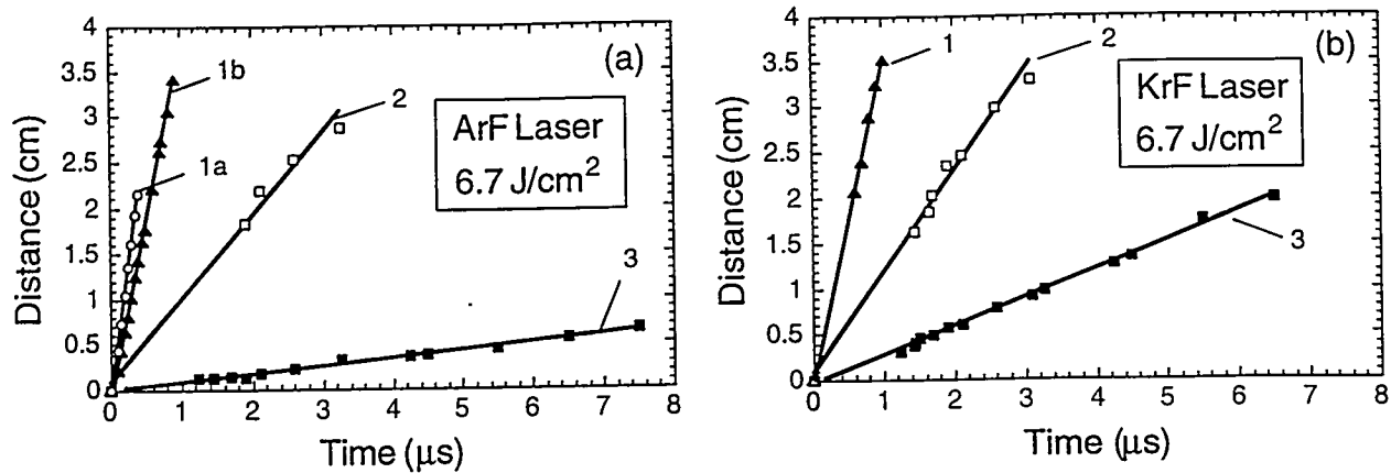
Fig.3. (a) R-t (distance versus time) plots of the propagation of the 1st, 2nd and 3rd plasma components along the normal to the pyrolytic graphite target in vacuum following ArF-laser (6.7 J/cm 2 ) ablation [see Figs.1(c), 1(d), and Fig. 2]. The lines labeled 1b (slope 3.9 cm/μs), 2 (slope 0.9 cm/μs) and 3 (slope 0.08 cm/μs) correspond to linear fits of the propagation emission intensity maxima positions for the 1st, 2nd and 3rd plasma components, respectively. The line 1a (slope 5.5 cm/μs) traces the position of the leading edge (defined as 10% of the maximum emission intensity) of the first component. (b) Propagation of the 1st (slope 3.5 cm/μs), 2nd (slope 1.1 cm/μs) and 3rd (slope 0.3 cm/μs) plasma components for the KrF-laser (6.7 J/cm 2 ) generated plasma [see Fig.1 (b)].
