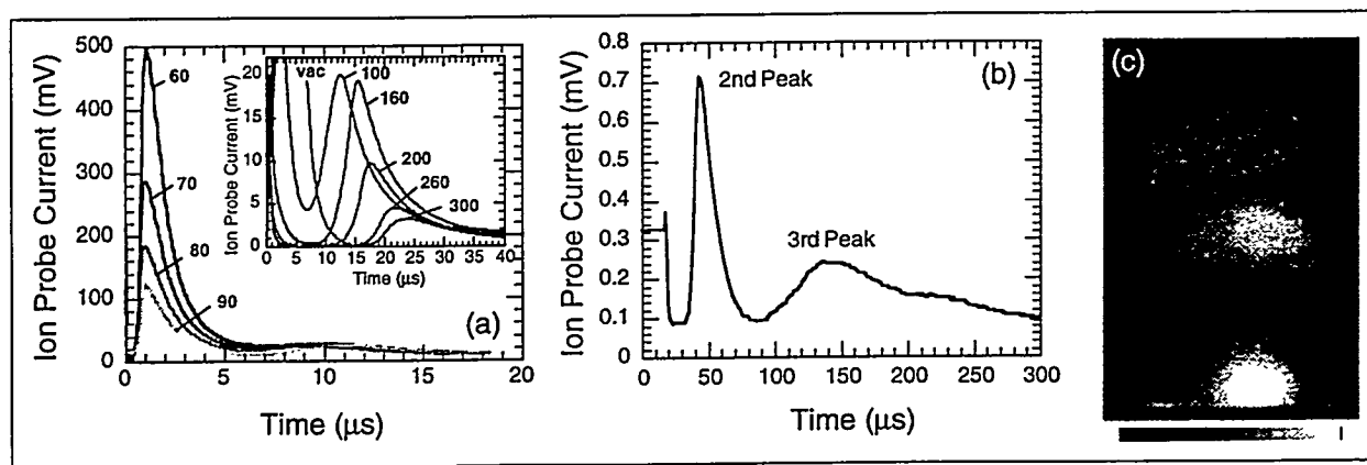
Fig. 7. (a) Ion probe current (mV into 50\text{ }\Omega ) induced by the ArF-laser ( 7\text{ J}/\text{cm}^2 ) generated plasma at d = 5\text{ cm} along the normal to the graphite target into 60, 70, 80 and 90 mTorr of Ar. In addition to the dominant fast component of the ion flux, a second component is observable at delays of \sim 10\text{ }\mu\text{s} . The insert shows the disappearance of the fast component and the evolution of the second component for vacuum ( 7 \times 10^{-7}\text{ Torr} ) and argon pressures of 100, 160, 200, 260, and 300 mTorr. (b) Ion current versus time after laser pulse in 350 mTorr of Ar. (c) ICCD image of luminescence (unfiltered) from the ArF-laser ( 6.0\text{ J}/\text{cm}^2 ) generated carbon plasma propagating into 70 mTorr of argon ( 2.1\text{ }\mu\text{s} delay, 0.2\text{ }\mu\text{s} exposure). The grayscale palette used is shown.
