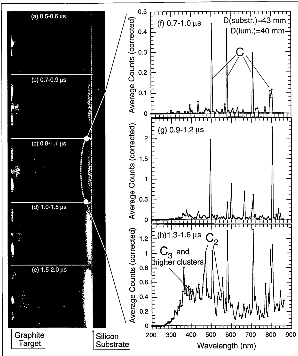
Fig. 6. (a)-(e) Species-resolved ( \lambda = 470 \text{ nm} \pm 5 \text{ nm} , \text{C}_2 Swan band emission) gated-ICCD images tracing the evolution of the near-substrate luminescence caused by the collision of the KrF-laser ( 17.7 \text{ J/cm}^2 ) carbon plasma plume with an unheated Si (100) substrate in vacuum. The substrate is located at the thin dashed line. Also shown is the propagation of the 'footprint' luminescence along the target surface and the forward-expanding 3rd component at the left of the frame. The emission spectra at d = 4.0 \text{ cm} (3 mm above the substrate surface) of the forming 'rebound' luminescence are given during (f) 0.7–1.0 \mu\text{s} , (g) 0.9–1.2 \mu\text{s} and (h) 1.3–1.6 \mu\text{s} , respectively. Arrival of the atomic 2nd component in (f) leads to the gas-phase formation of \text{C}_2 and \text{C}_3 above the substrate surface as evidenced by the emission spectrum (h), which is remarkably similar to that of the slow-moving 3rd component back near the target surface [see Fig. 5(a) and 5(b)].
