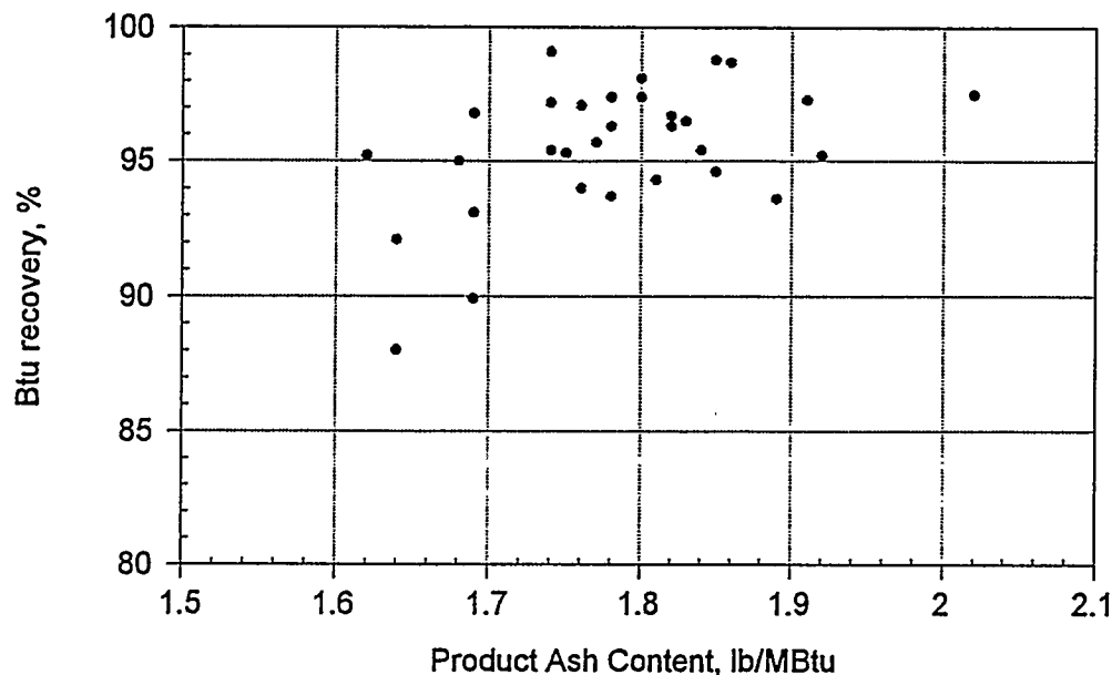
Figure 10. Elkhorn Agglomeration - Product Ash vs Btu Recovery
