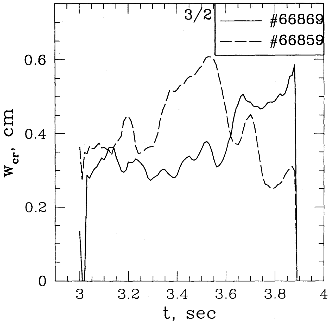
FIG. 2. Comparison of the calculated threshold width evolution w_{cr}(t) for the tearing mode 3/2 in two similar TFTR discharges #66869, and #66859. In one of them #66869 3/2 tearing mode-like MHD activity was observed.
