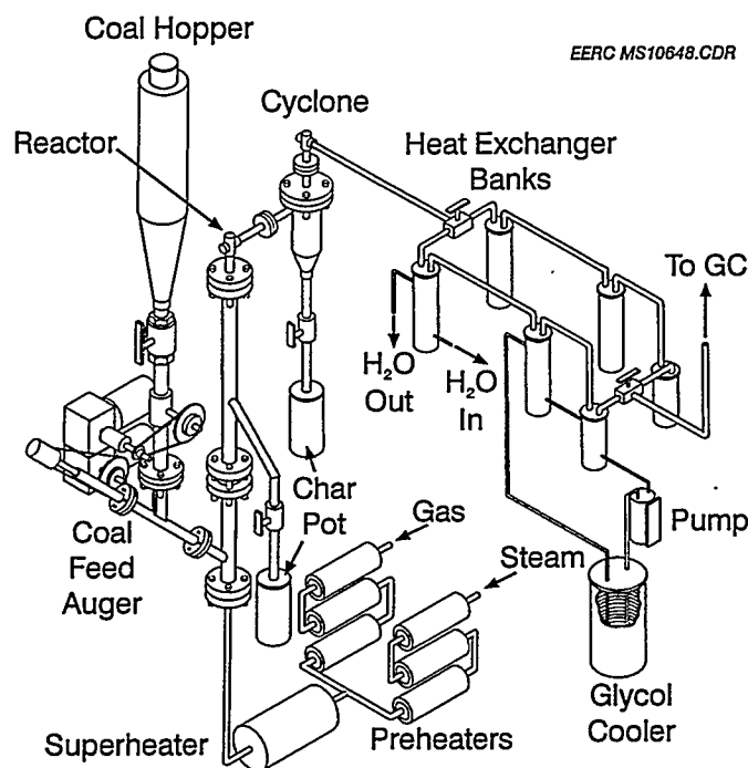
Figure 1. 4-lb/hr CFBR.
