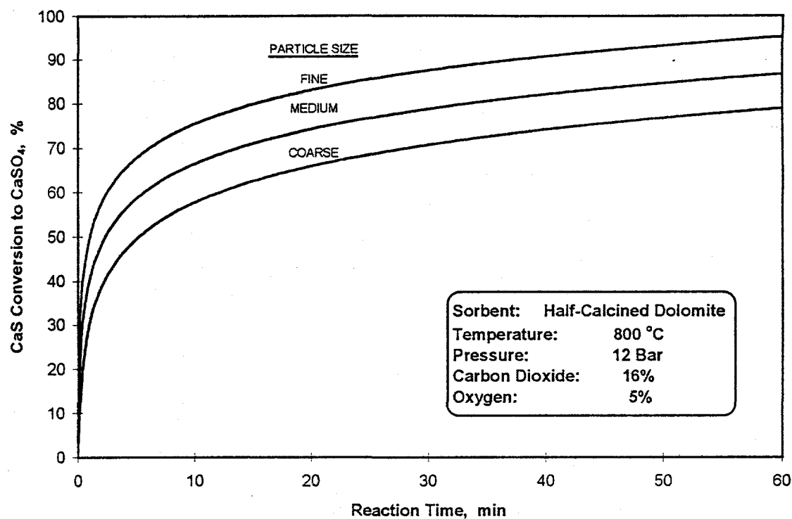
Figure 7. EFFECT OF SORBENT PARTICLE SIZE ON THE SULFATION REACTION RATE (16% CO 2 ).
