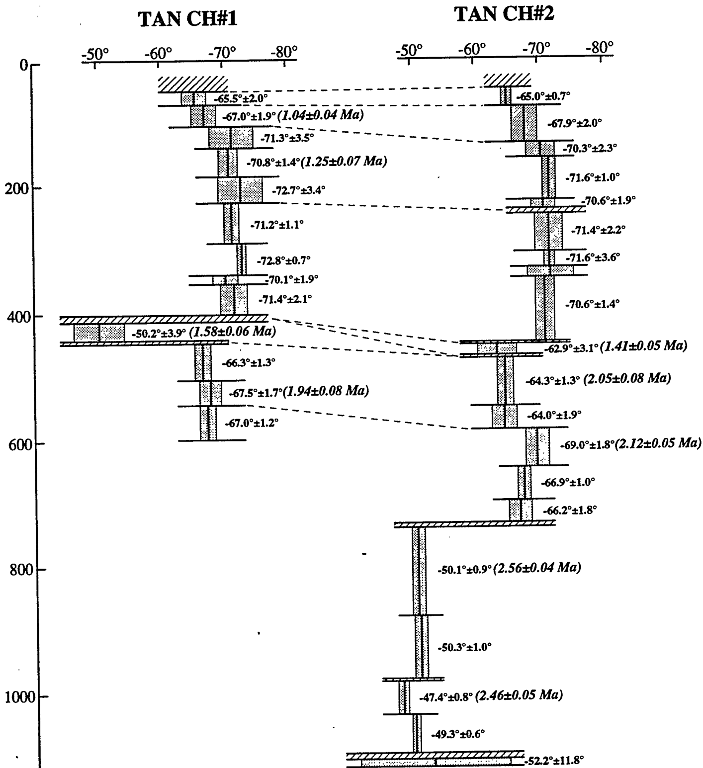
Figure 2. Simplified log of core stratigraphy, K-Ar ages (in parentheses), and paleomagnetic inclination data in wells TAN CH#1 and TAN CH#2. Diagonal ruling indicates sedimentary interbeds, horizontal lines are flow contacts, and light stippling pattern represents 95% confidence limits around the mean inclination values. Dashed lines represent correlations based on paleomagnetic and petrographic data described in this report.
