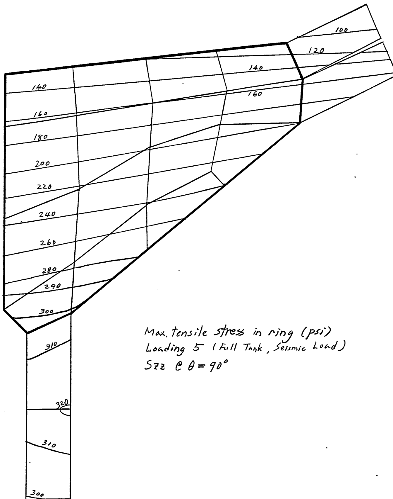
Fig. 2. Maximum Tensile Stress Distribution in Ring
