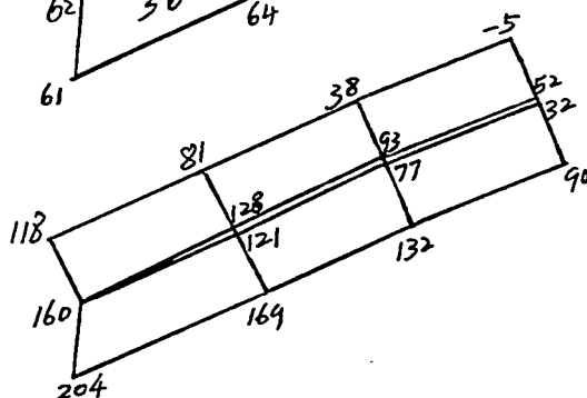
Stresses S_{xx} psi + tension - compression
