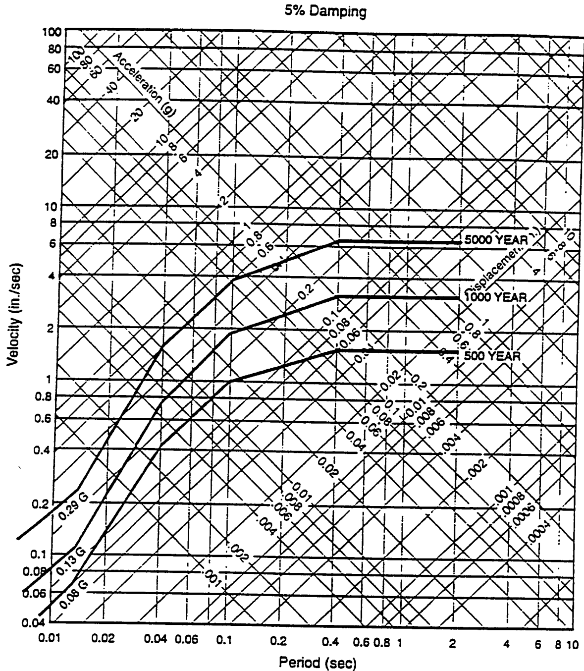
OAK RIDGE - SITE SPECIFIC UNIFORM HAZARD RESPONSE SPECTRA FOR HORIZONTAL ROCK MOTION
