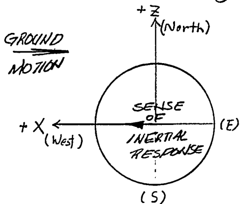
Earthquake Load on Tank
