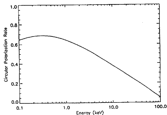
Figure 3. Calculated circular polarization of the EMW
