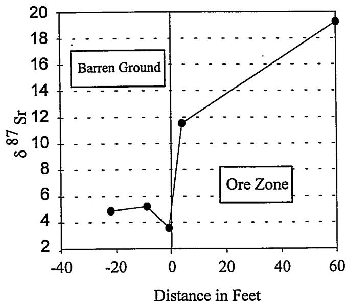
Figure 6 Variation of \delta^{87}\text{Sr}_i in Bonanza King Formation across the contact of an ore shoot in the Sterling Mine.
