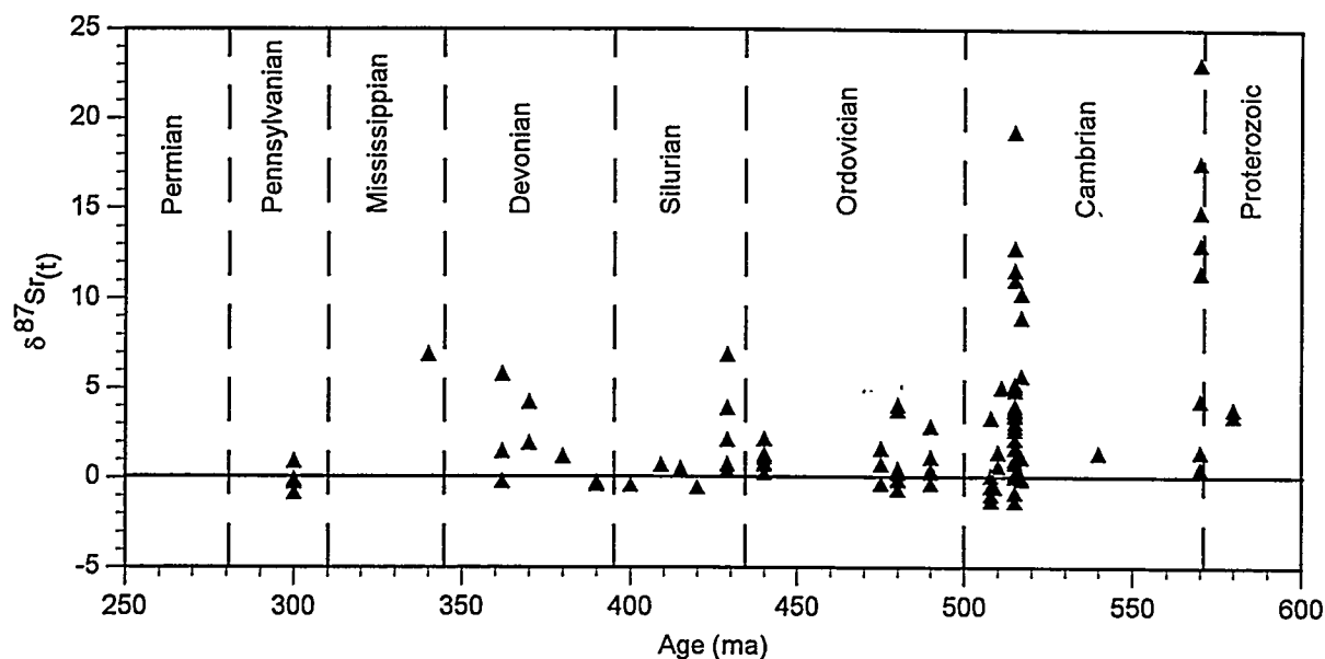
Figure 3 \delta^{87}\text{Sr}_r values for samples as a function of their age (see text for definition of \delta^{87}\text{Sr}_r ).
