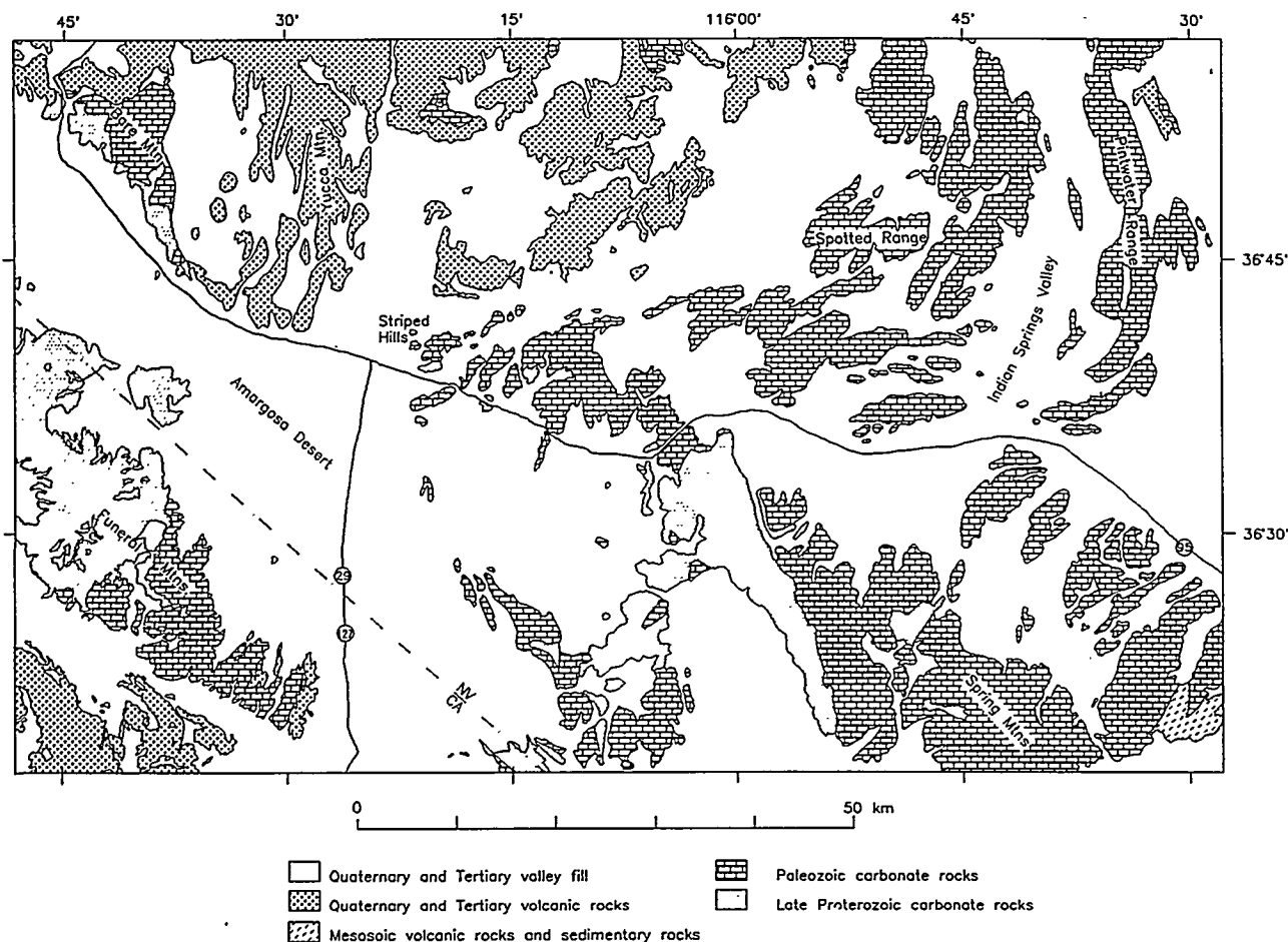
Figure 1 Regional geologic sketch map.
