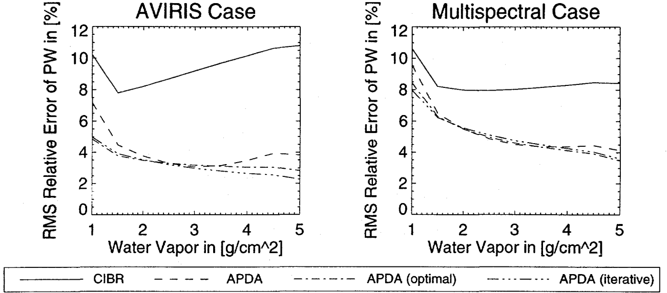
Figure 2: RMS relative error \epsilon(PW_j) in % in water vapor for all 379 reflectance spectra as a function of water vapor for four different water vapor retrieval techniques.
