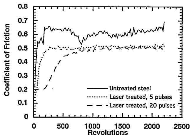
Figure 2. Friction as a function of number of revolutions for the untreated surfaces and samples treated with 5 and 20 pulses of excimer laser radiation at 1.1 \text{ J-cm}^{-2} (samples I, II, and III). The duration of the initial low friction period is precisely related to the number of pulses.
