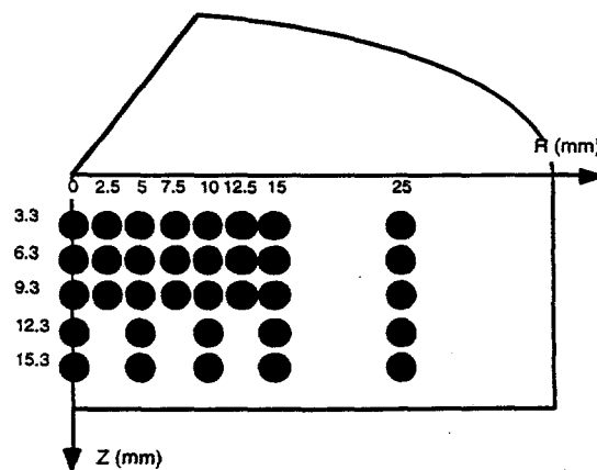
Figure 2 Neutron diffraction measurement locations
