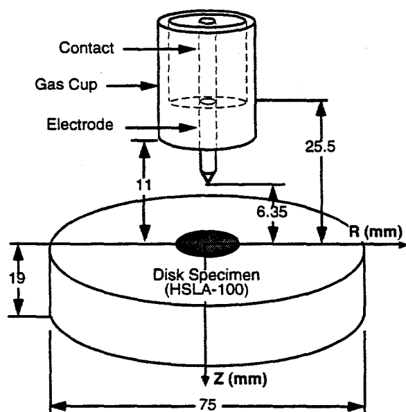
Figure 1 Welding setup.
