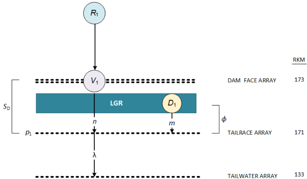
Figure 2.3. Schematic of the ViRDCt Release-Recapture Model to Estimate Dam Passage Survival at LGR in 2018. Alive ( R_1 ), virtual ( V_1 ), and dead fish ( D_1 ) releases are denoted, along with hydrophone detection arrays. Schematic a) allows dead fish detection at both the tailrace and tailwater arrays, and b) permits dead fish detection at the tailrace only.
