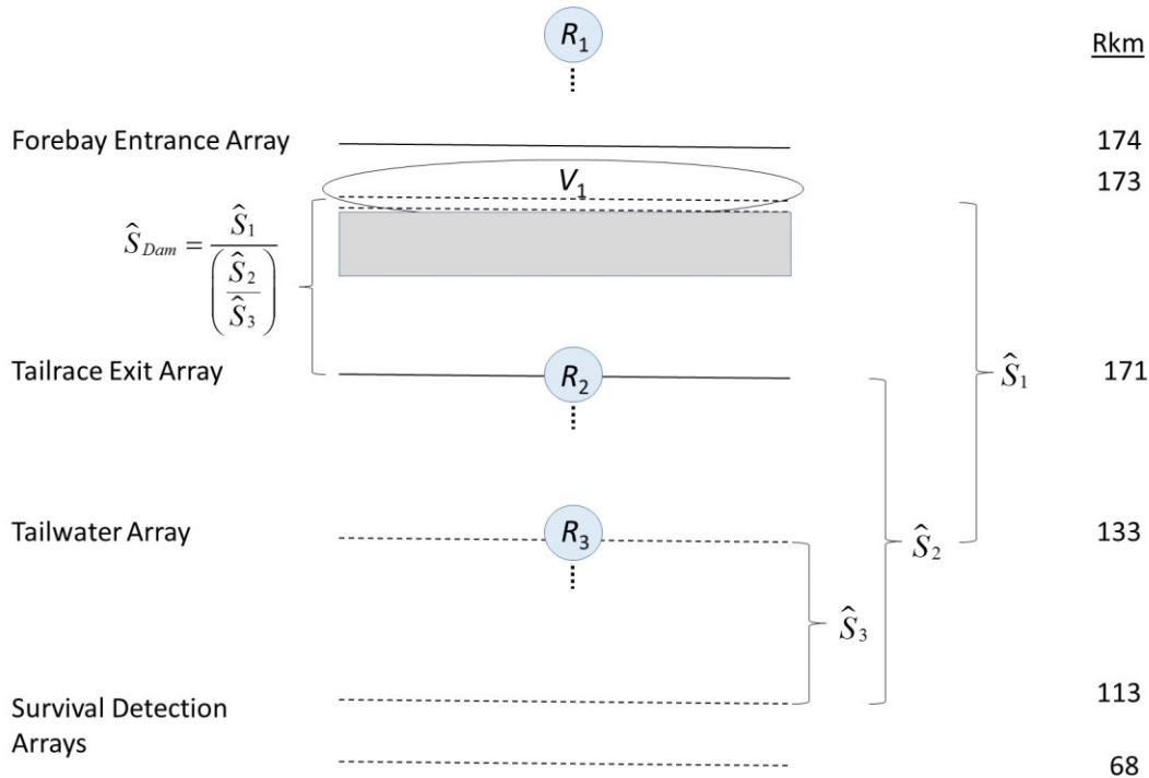
Figure 2.1. Virtual/Paired-Release-Recapture Design to Estimate Dam Passage Survival at LGR in 2018. Release groups R_1 , R_2 , and R_3 are denoted, along with the virtual release V_1 created at the face of the dam and associated hydrophone detection arrays and survival parameters.
