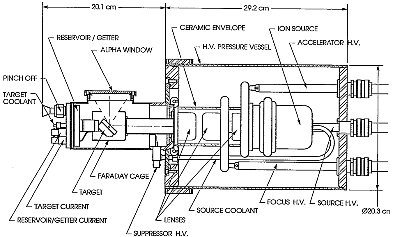
Fig. 7. Design drawing of accelerator head for new advanced APSTNG being constructed by MF Physics.
