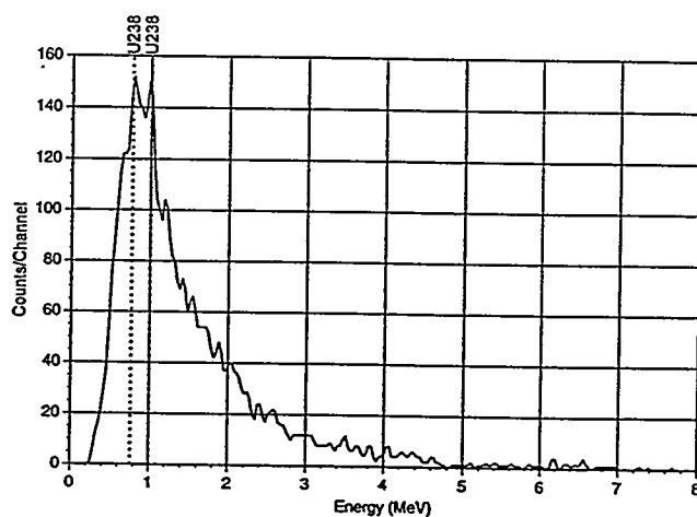
Fig. 4. EGRIS energy spectrum measured for U-238 fission.
