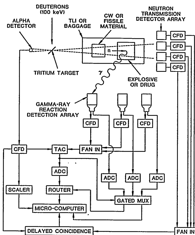
Fig. 1. Schematic layout of "general purpose" APSTNG-based interrogation system, with EGRIS and FNTI modes.
