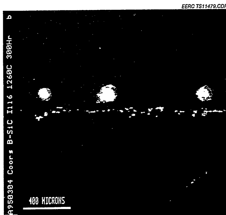
Figure 1. SEM photo showing the cross section through the Coors \beta -SiC exposed to the Illinois No. 6 slag. Circular iron silicides are present along the slag-ceramic interface.
