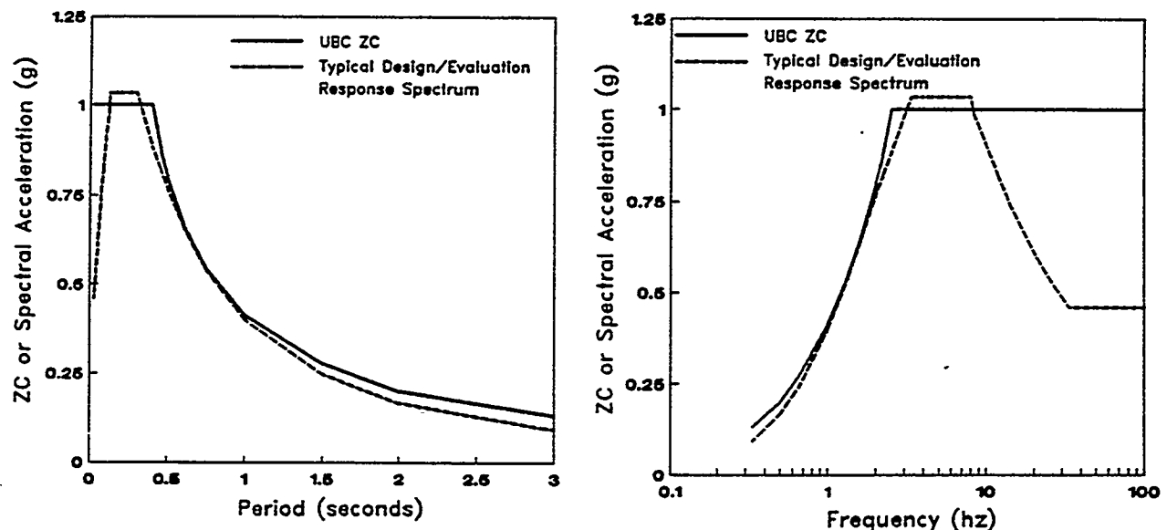
Figure C-10 Comparison of UBC ZC with Typical Design/Evaluation Response Spectrum
