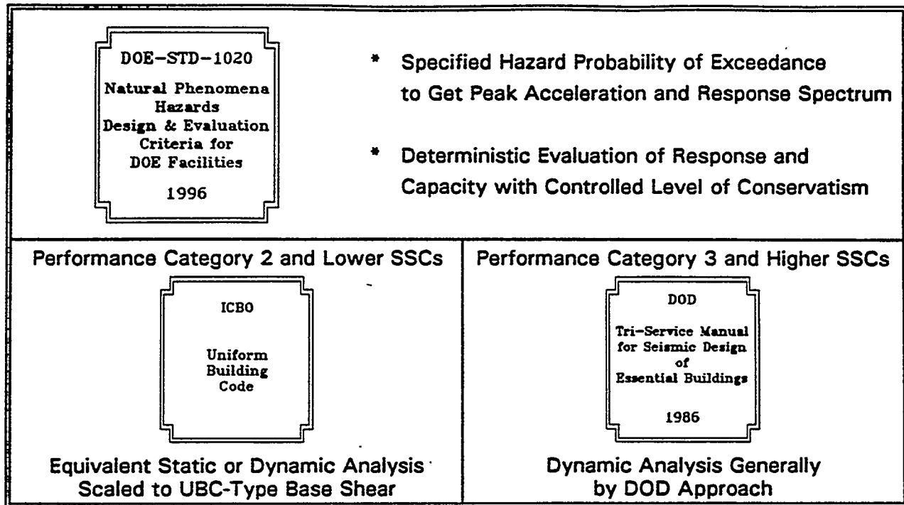
Figure C-12 Earthquake Provisions Basic Approach
