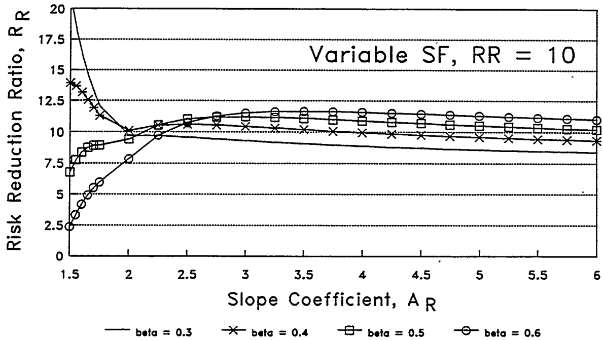
Figure C-7 Value of R_R vs A_R for Variable SF (Fig. C-5 for PC 4)
