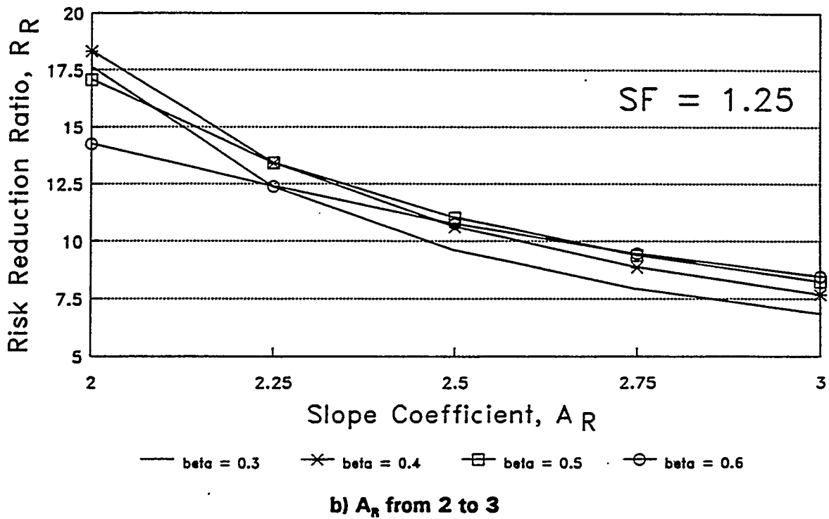
Figure C-4 Value of R_R vs A_R for SF = 1.25 (PC 4)
