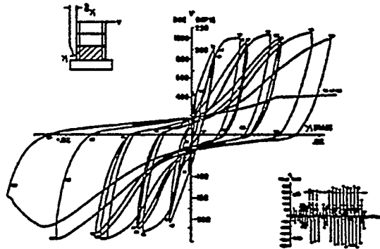
a. Shear force-distortion for concrete wall test (Ref. C-18)
