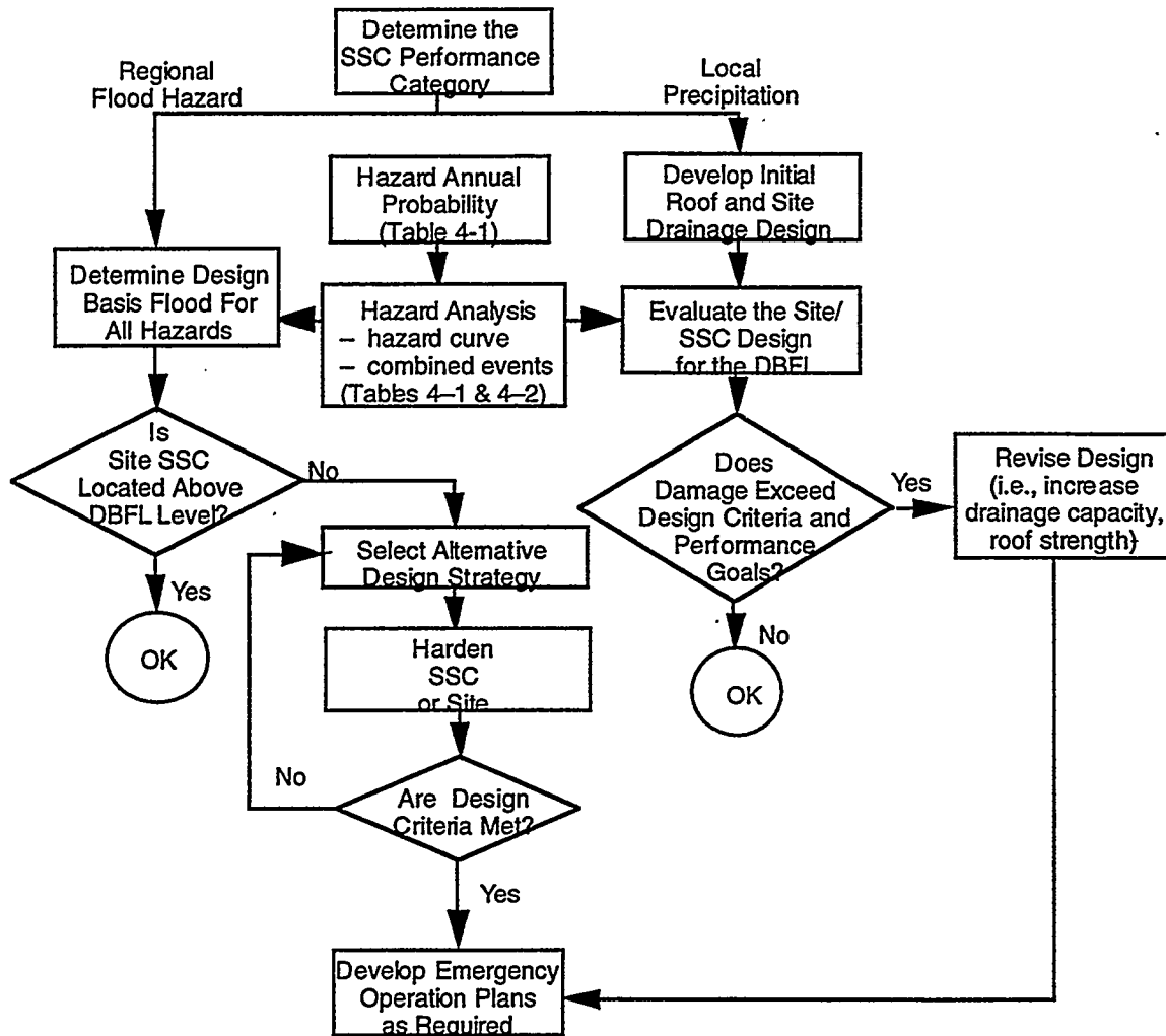
Figure 4-1 Flood Evaluation Process
