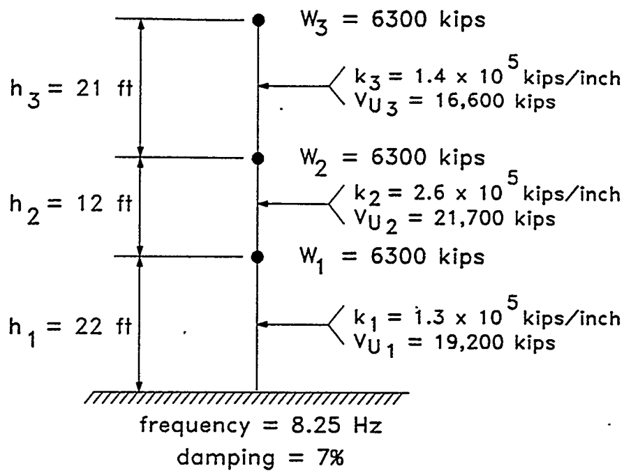
Figure C-14 Three Story Shear Wall Structure
