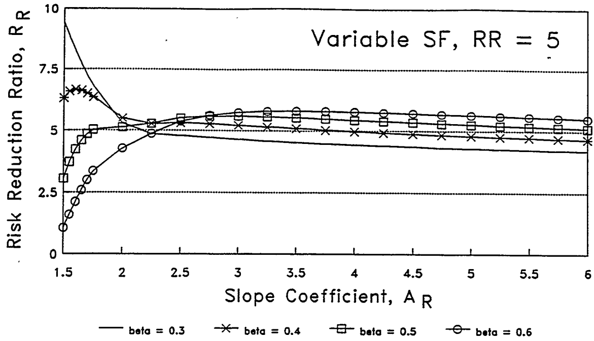
Figure C-6 Value of R_R vs A_R for Variable SF (Fig. C-5 for PC 3)
