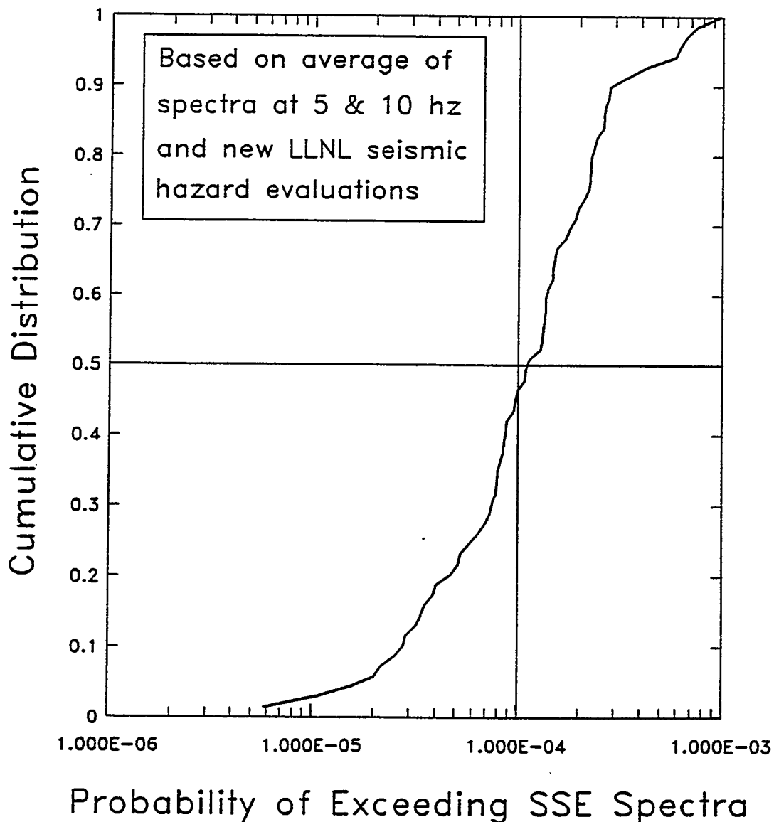
Figure C-9 Probability of Exceeding SSE Response Spectra
