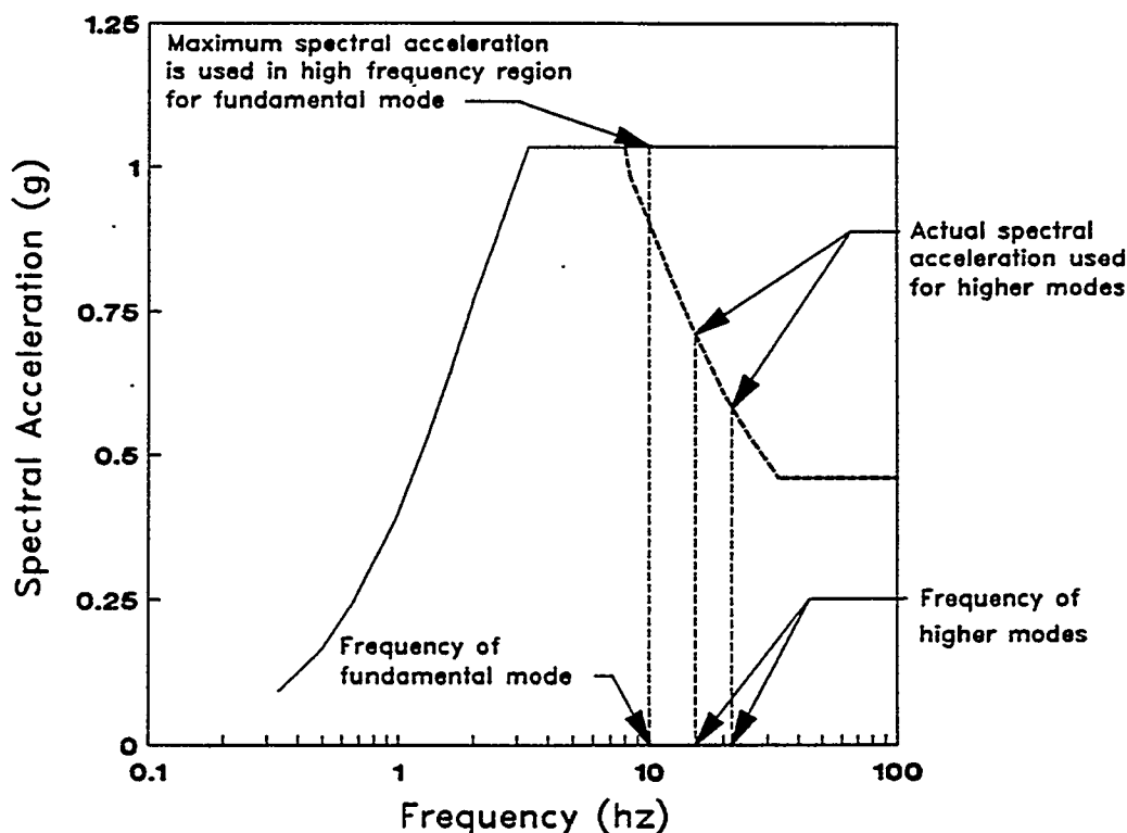
Figure C-11 Spectral Acceleration in the High Frequency Region for an Example Design/Evaluation Ground Response Spectrum
