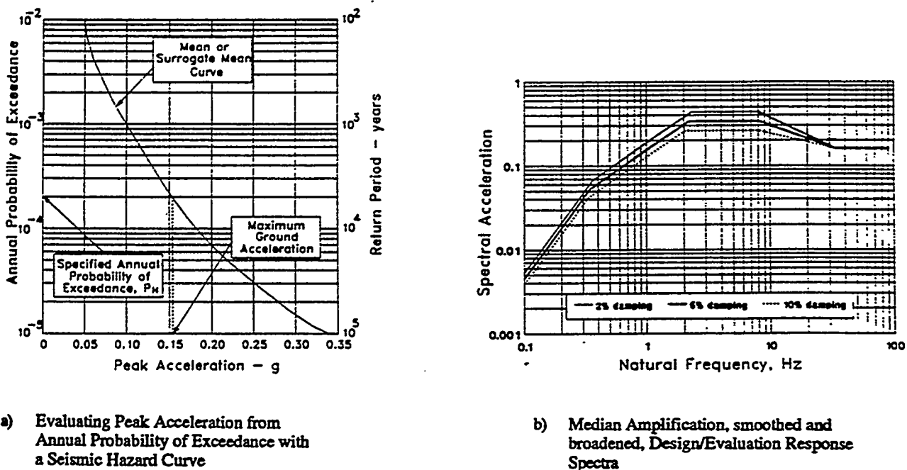
Figure 2-2. Earthquake Input Excitation is Defined by Maximum Ground Acceleration Anchoring Site-Specific Response Spectra
