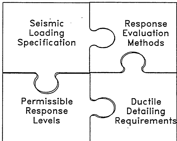
Figure C-1 Consistent Specification of All Seismic Design/Evaluation Criteria Elements
