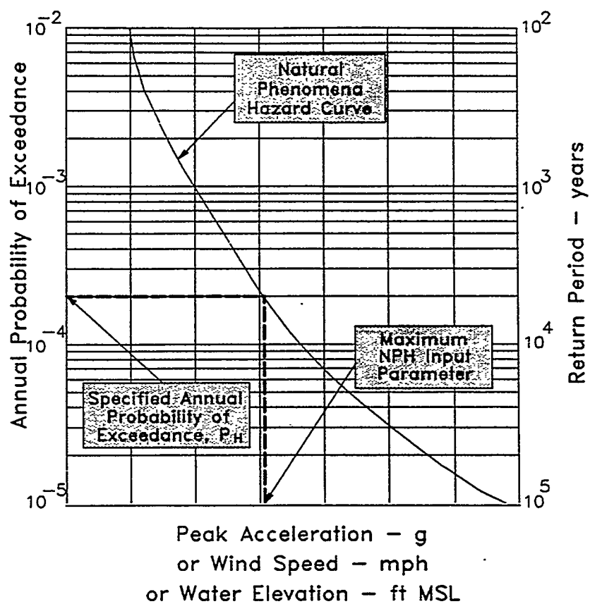
Figure A-1 Example Probabilistic Natural Phenomena Hazard Curve
