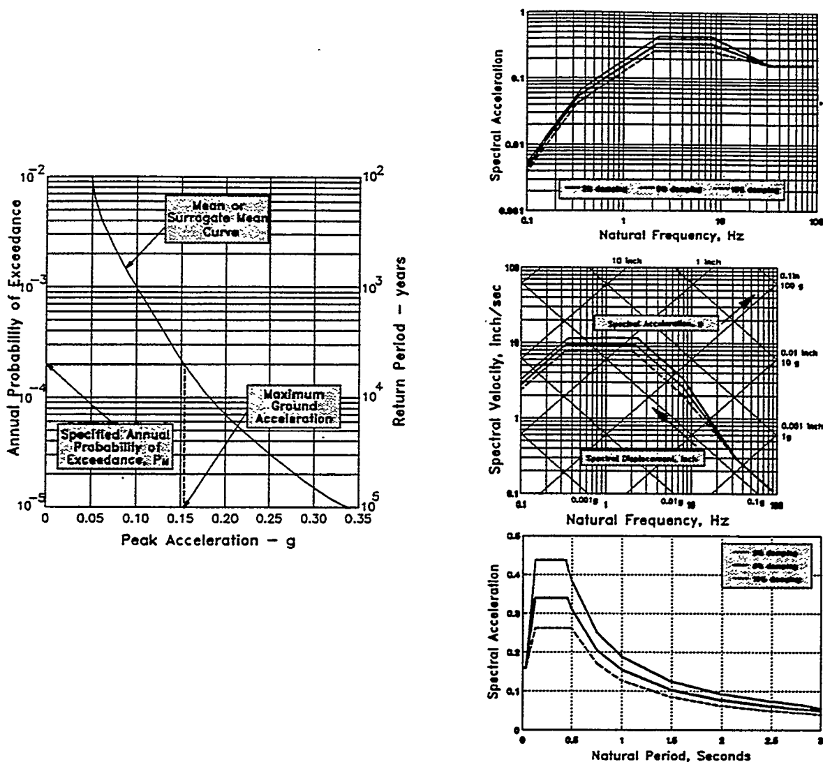
Figure C-8 Earthquake Input Excitation is Defined by Maximum Ground Acceleration Anchoring Site-Specific Response Spectra
