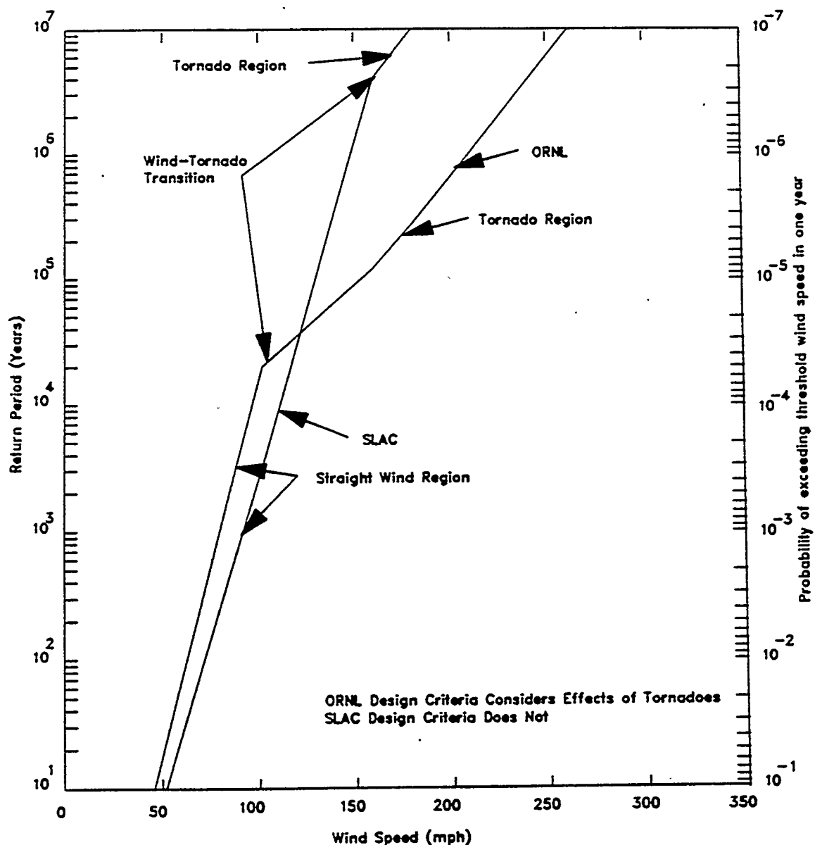
Figure D-1 Straight Wind and Tornado Regions of Wind Hazard Curves
