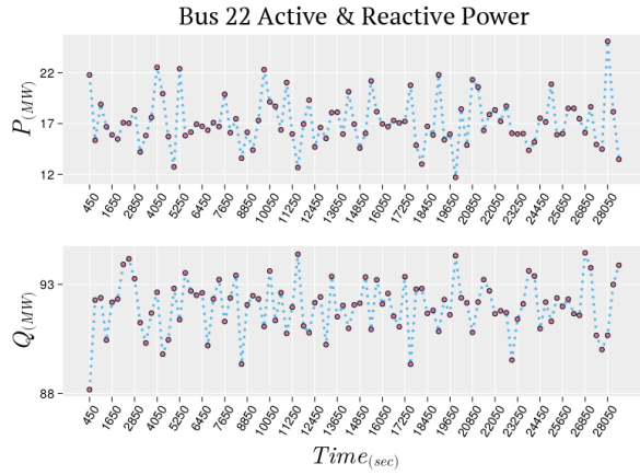
Fig. 7: Bus 22's active (P) and reactive (Q) power levels after steady state convergence over simulation time. This bus has the injection of WEC 2.
