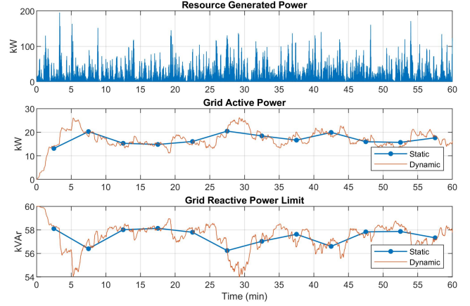
Fig. 4: Example output of the W2W Simulink model.
