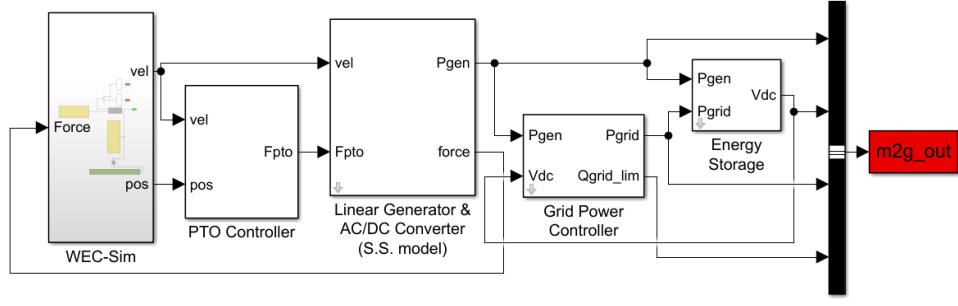
Fig. 3: Wave-to-Wire system diagram in Simulink.
