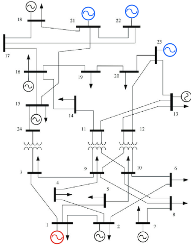
Fig. 5: One-line diagram of the IEEE RTS 96 bus test case (Area 1). The red generator indicates the swing bus. The blue generators at Buses 21, 22, and 23 represent the WECs that replace the traditional generators at those buses.
