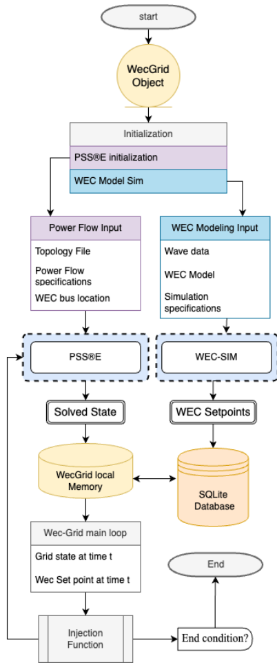
Fig. 1: The flow chart pipeline illustrates the end-to-end processing of the WEC model integration of steady state power flows. One of the software's key features is its modularity and use of open-source power flow solvers and WEC modelers. The dotted boxes indicate that the blocks (PSS®E and WEC-SIM) can be substituted with support modeling software.
