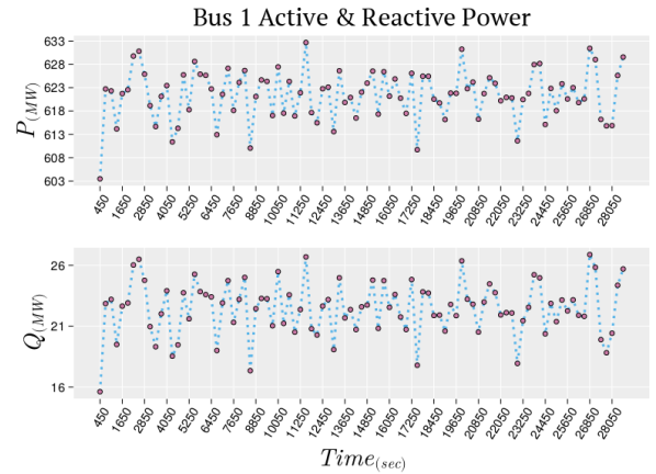
Fig. 6: Swing bus's active (P) and reactive (Q) power levels after steady state convergence over simulation time.
