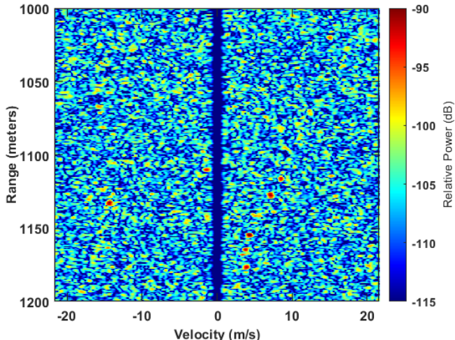
Fig. 6. Range-Doppler response for M = 10^4 unique segments of a “variable symbols” CE-OFDM signal that has uniform spacing and changes symbols every 100\ \mu\text{s}
