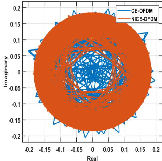
Fig. 7. Plot of the complex signal samples for NICE-OFDM and “variable symbols” CE-OFDM after loopback capture, illustrating the relative distortion that each experience (ideally each would remain on the unit phase circle)
