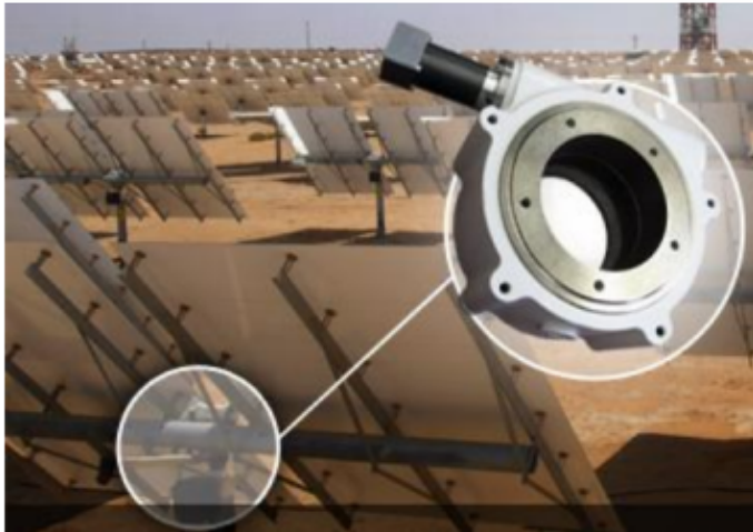
Azimuth drive with worm-gear – a typical standard solution. Source: (Conedrive, 2013)
