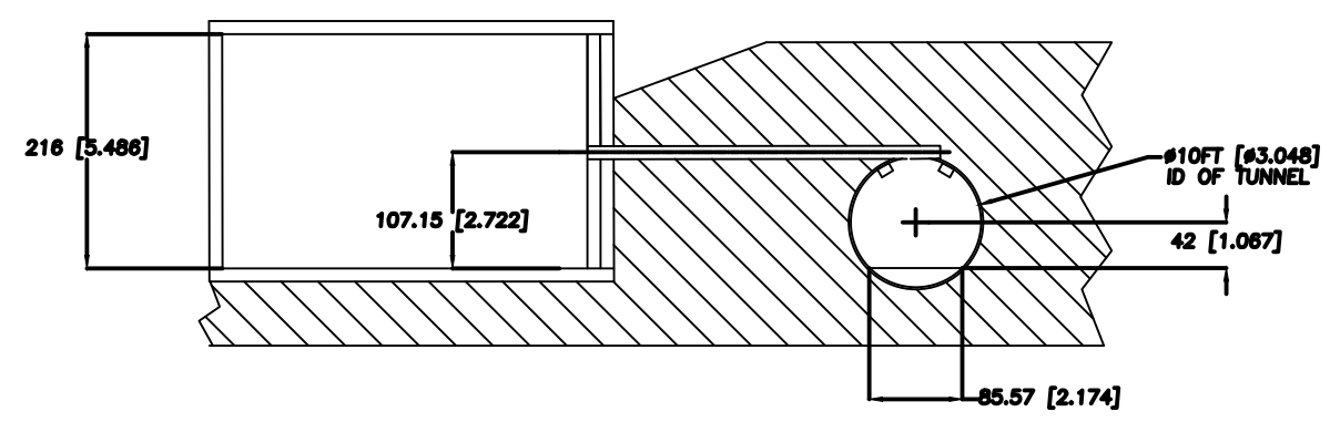
SECTION A-A VIEW ROTATED 90° CLOCKWISE
