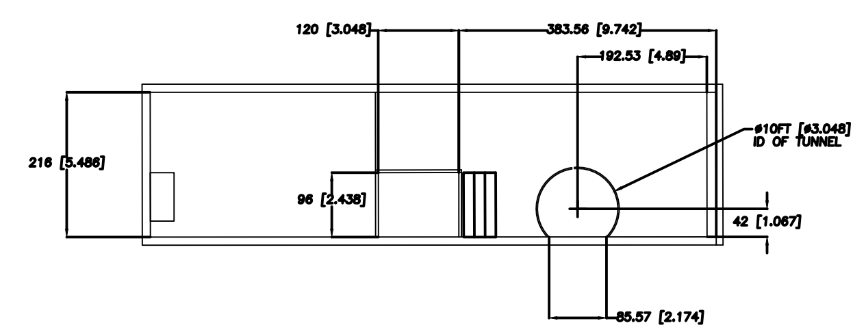
SECTION B-B VIEW ROTATED 90° CLOCKWISE
