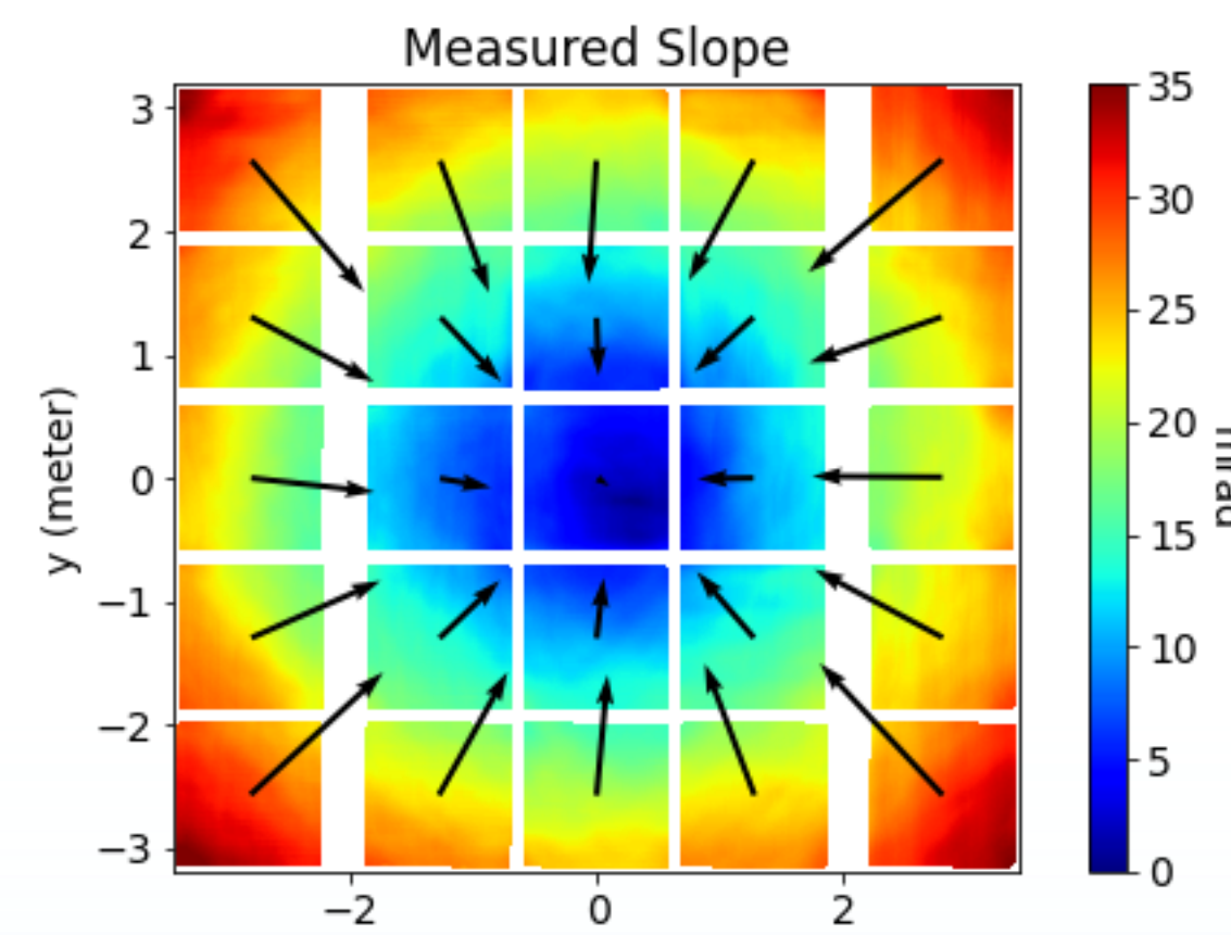
Measured slope magnitude with arrows showing facet canting.
