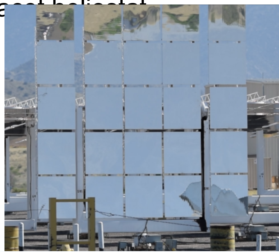
Multifacet heliostat measured by SOFAST
