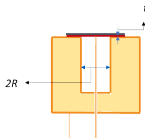
Figure 2. Gardon gauge construction, with parameters to be varied. Colors correspond to materials used, copper (orange), constantan (red) and coating (black).
