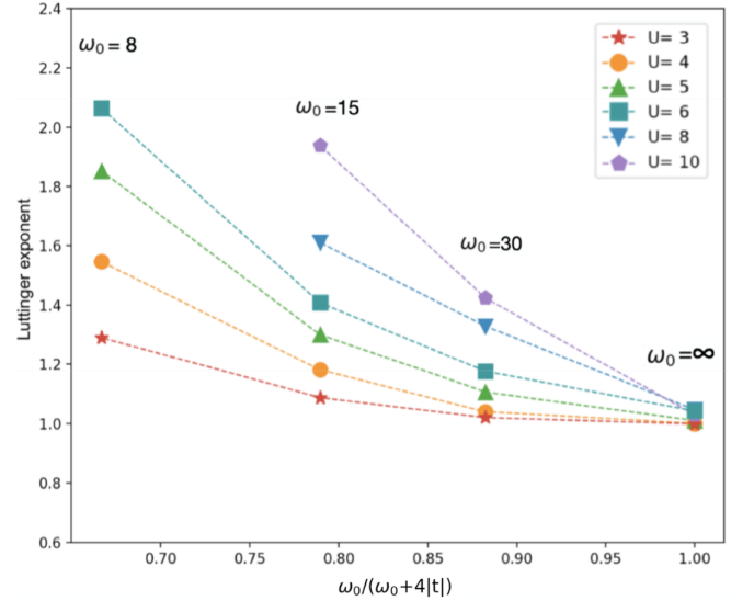
FIG. 5: A summary of Luttinger exponents for all values of (U, \omega_0) that have been calculated by DMRG.
