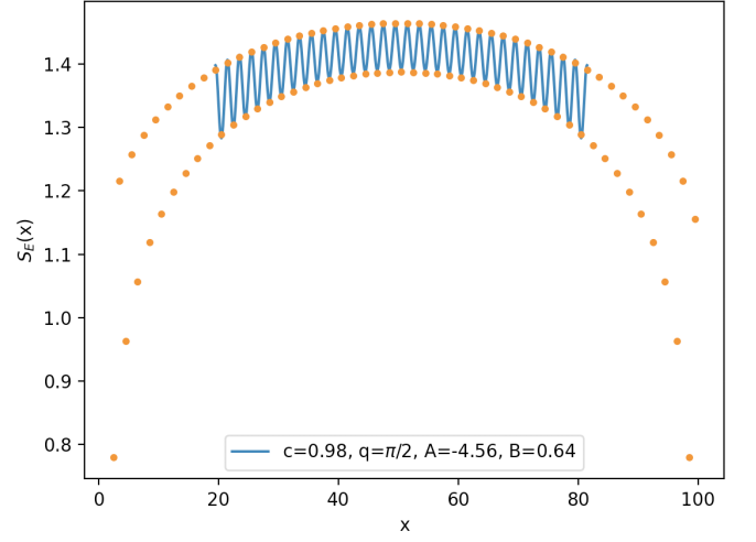
FIG. 7: Here use U = 3 and \omega_0 = 8 as an example. We fit the middle part of the system with Eq.(8) as shown by the solid blue line. The extracted values of parameters are shown in the legend.
