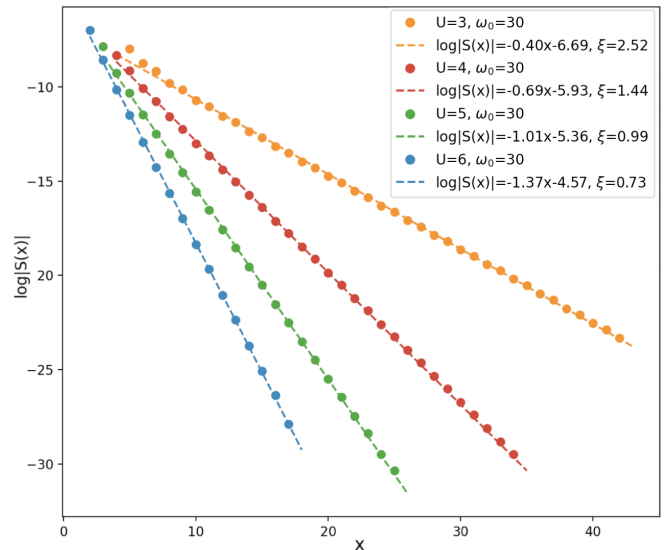
FIG. 2: Spin-spin correlations Eq. 5 with exponential fit.
