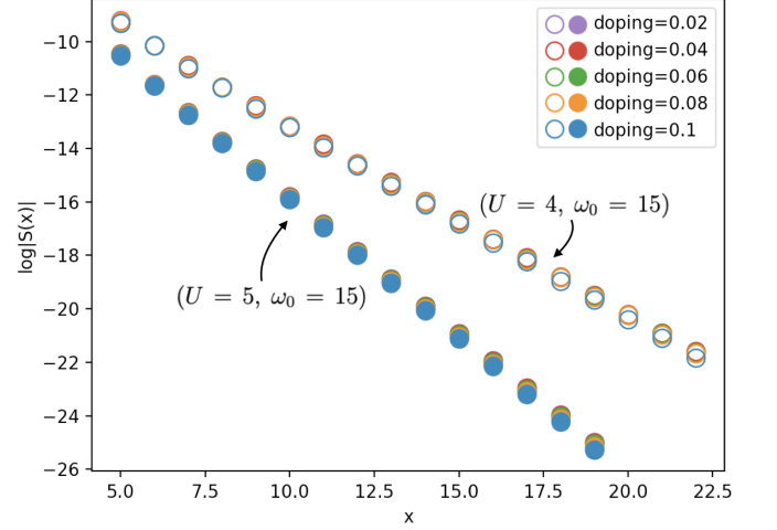
FIG. 9: Spin-spin correlation for (U, \omega_0) = (4, 15) and (5, 15) at different hole doping concentration from 0.02 to 0.1. We see for both values of (U, \omega_0) , the spin correlations are essentially unchanged at different doping.
