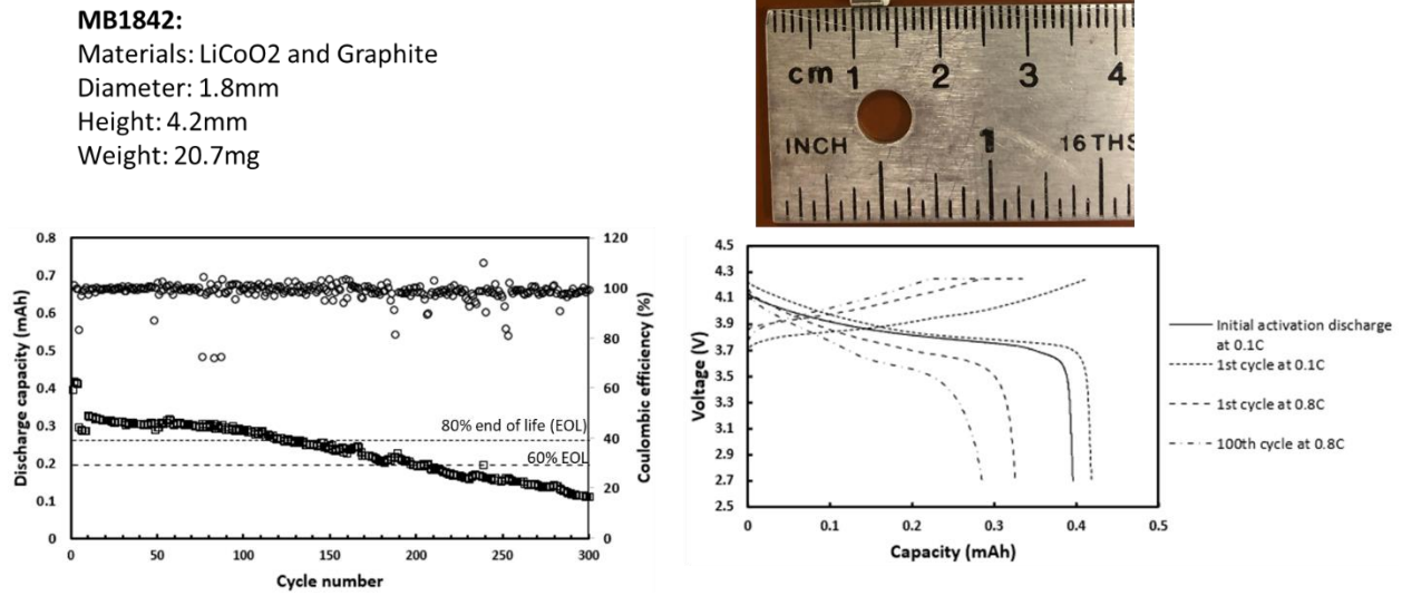
Fig.2 Battery performance of the exemplified rechargeable micro-battery.
