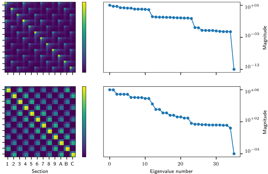
FIG. 4. Top row: Horizontal dimension, bottom row: vertical dimension. Left column: The 36 \times 36 matrix J^T J . The axes numbering indicates the 12 sections of SIS18 in hexadecimal notation and there are three rows/columns per section, corresponding to the F, D, and T quadrupoles (in that order) of each section. Right column: The eigenvalues of corresponding J^T J matrices. The color bars and eigenvalue magnitude indicate the magnitude of J^T J in units of \text{m}^4/\text{rad}^2 . The values of the color bar correspond to those of the eigenvalue plots shown on the vertical axes. For the horizontal dimension, the smallest eigenvalue \lambda_{35} is nonzero only due to limited floating point precision. When inspecting the 12 smallest horizontal eigenvalues, it can be observed that the \lambda_{24} and \lambda_{25} eigenvalues have a slightly greater magnitude than the remaining nine eigenvalues (neglecting \lambda_{35} ). These two eigenvalues correspond to sections 4 and 6 where the horizontal steerer is shifted by a few meters compared to the other sections.
