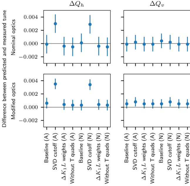
FIG. 14. Difference between predicted and measured tunes for the various optics and inverse modeling methods. Top: \Delta Q_h , \Delta Q_v for nominal extraction optics. Bottom: \Delta Q_h , \Delta Q_v for the modified optics. The different methods are indicated on the horizontal axis and are the same for each subplot. (A) and (N) denote, respectively, the usage of analytical and numerical Jacobian. The vertical bars indicate the measurement uncertainty.
