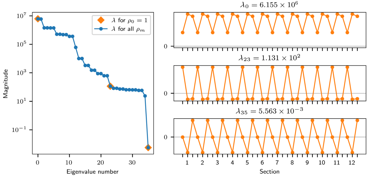
FIG. 7. Globally symmetric eigenmodes of J^T J in vertical dimension which arise due to the fact that the vertical lattice is symmetric from section to section. Each tick marker on the horizontal axis of the eigenvector plots indicates a quadrupole (F, D, and T quadrupole per section).
