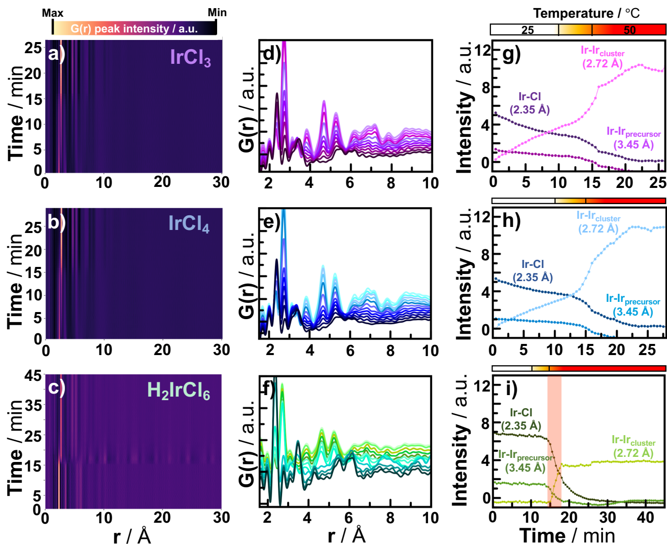
Figure 1. (a-c) Experimental in situ X-ray TS data following the formation of Ir NPs from (a) \text{IrCl}_3 , (b) \text{IrCl}_4 and (c) \text{H}_2\text{IrCl}_6 as precursors presented in real space, G(r) . (d-f) Selected PDFs from (bottom) precursor to (top) Ir NPs from the beginning to the end of the experiments with 2.5 min time resolution. (g-i) Evolution of PDF peak intensity associated with Ir-Cl (2.35 Å), Ir-Ir in the precursor (3.45 Å) and Ir-Ir in the NPs formed (2.72 Å). Panels (a, d, g) relate to \text{IrCl}_3 , (b, e, h) relate to \text{IrCl}_4 and (c, f, i) relate to \text{H}_2\text{IrCl}_6 .
