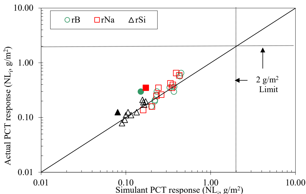
Figure 1.1. Comparison of PCT responses (normalized loss, NL_i , \text{g}\cdot\text{m}^{-2} ) for radioactive actual and non-radioactive simulated LAW glasses. The solid symbols represent AN-102 PCT responses discussed in the text. (Vienna, 2004)
