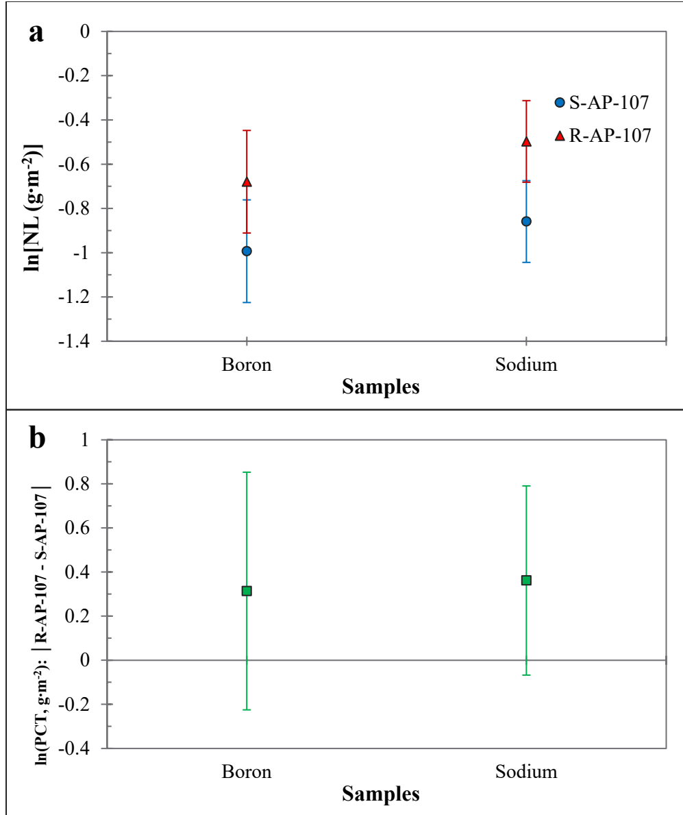
Figure 4.1. a) average \ln[NL_i, \text{g}\cdot\text{m}^{-2}] boron and sodium responses for S-AP-107 and R-AP-107. Uncertainty is represented by SD_{i,pooled} values from Vienna et al. (2022). b) differences of S-AP-107 and R-AP-107 average \ln[NL_i, \text{g}\cdot\text{m}^{-2}] boron and sodium responses respectively. Uncertainties are associated with 90% confidence intervals ( U_{90\% \text{ CI, PCT}} ) as described in Equation 4.1.
