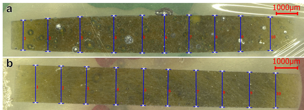
Figure 3.2. Examples of VHT cross section measurements: a) R-AP-107-VHT-c and b) S-AP-107-VHT-a.
