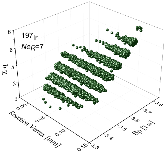
FIG. 4: LISE ++ 3D Monte Carlo calculations of the charge state distribution for 197 Ir versus the depth in the target at which the reaction occurs, assuming post-reaction charge state is Z - q = 7 . The charge state model GLOBAL was used.
