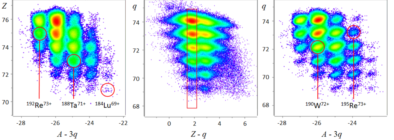
FIG. 2: Particle identification spectra obtained from D4b settings (see Table I). The separation of charge states is demonstrated in the Z - q spectra (center) where helium-like and lithium-like charge states were observed. The charge state selection gate at Z - q = 2 (red) is applied to both left and right plots. The Z vs. A - 3q (left) and q vs. A - 3q (right) spectra demonstrate mass, ion charge, and elemental separation quality. A \gamma -ray spectrum observed in coincidence with ^{190}\text{W}^{72+} ions labeled here was used to confirm the identification (Figure 3).
