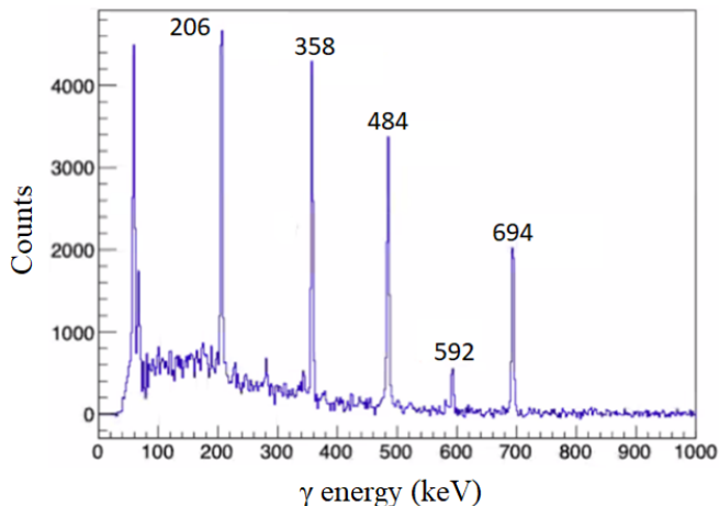
FIG. 3: A \gamma -ray spectrum of events in GREYINA recorded up to 800 \mu\text{s} after events identified as ^{190}\text{W} . The energies of the observed peaks correspond to gamma transitions from the 166 \mu\text{s} isomeric state of ^{190}\text{W} [29], confirming particle identification.
