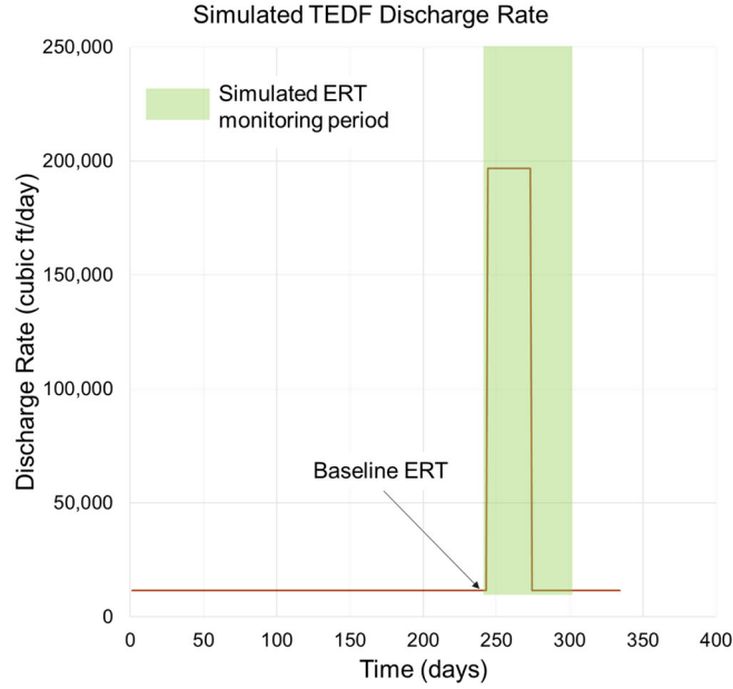
Figure 3. Simulated discharge rate.
