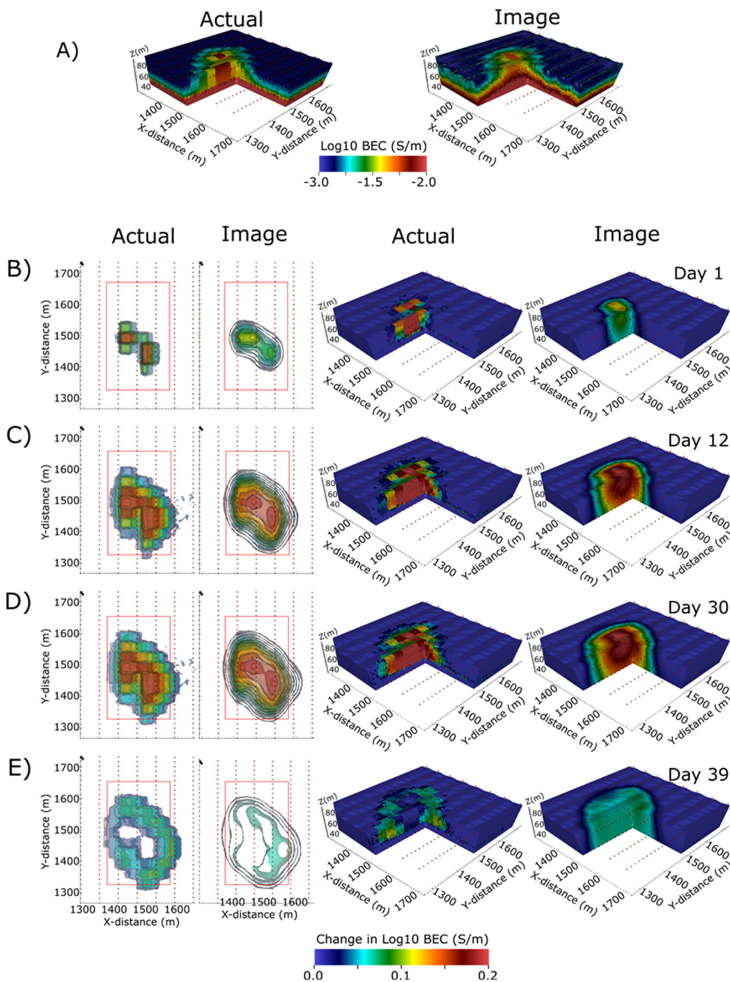
Figure 6. Summary results of ERT performance simulations. A) Actual and imaged baseline BEC after 243 day of infiltration at 11,500 ft 3 /d. B, C, D) Actual and imaged changes in BEC from baseline after 1, 12, and 30 days of infiltration at 197,000 ft 3 /d. E) Actual and imaged changes in BEC from baseline after 30 days of infiltration at 197,000 ft 3 /d followed by 9 days of infiltration at 11,500 ft 3 /d.
