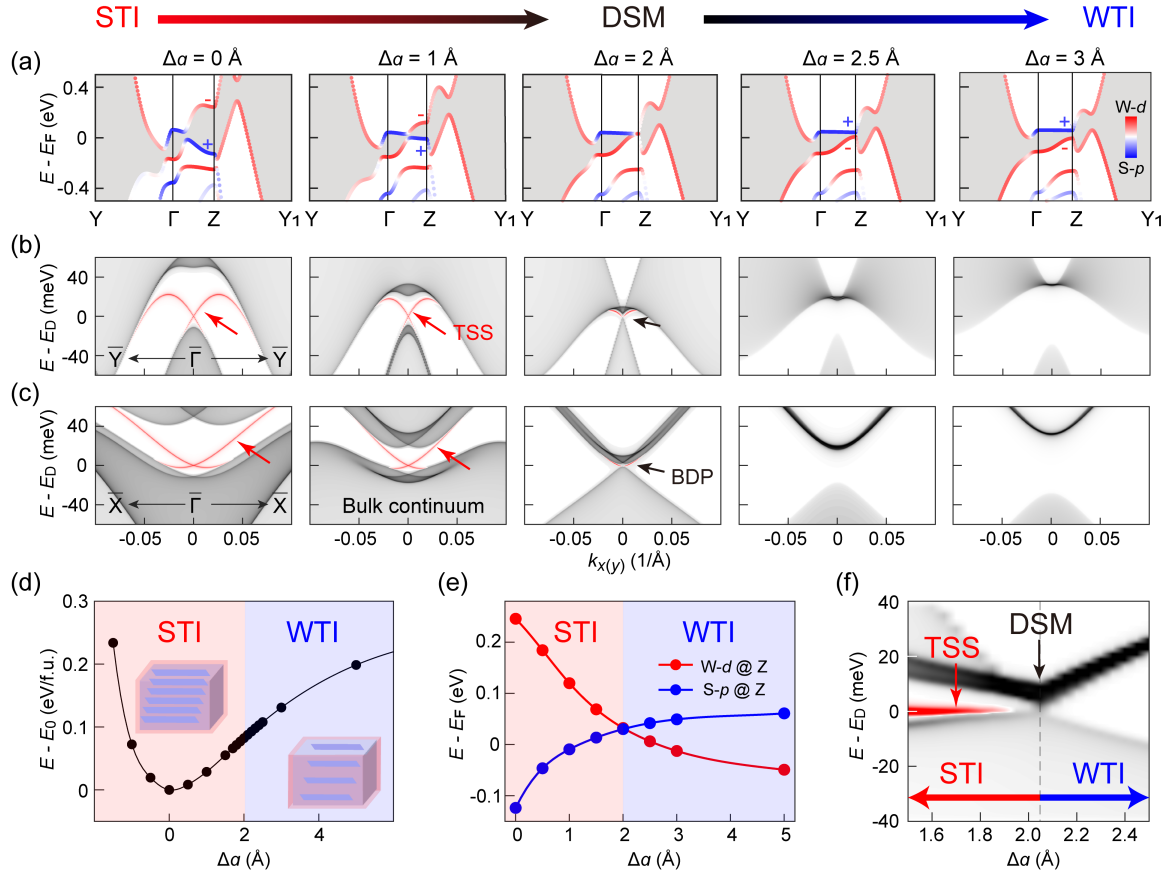
Figure 5. Calculated topological phase transition driven by the increasing interlayer distance.
