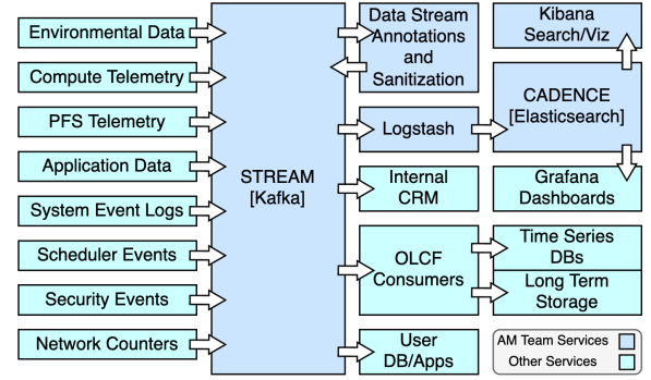
Fig. 1. STREAM is the narrow waist of OLCF's telemetry platform.
