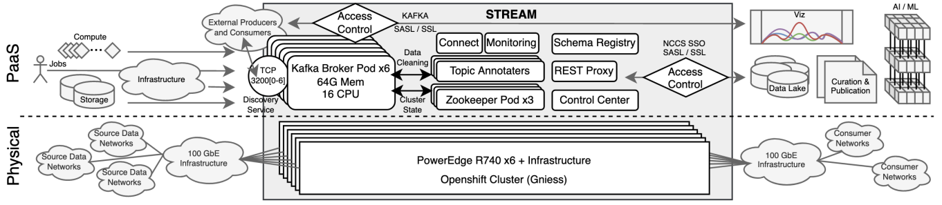
Fig. 2. Detailed STREAM components and their support by SLATE physical infrastructure. Data sources generally reside within their own network infrastructure on the left of the diagram while data sinks/destinations are on the right. SLATE also supports several data consumption applications.
