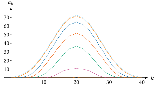
Figure 1: Graphical representation of the (KOH) summation with \ell = 8 and m = 5 .
