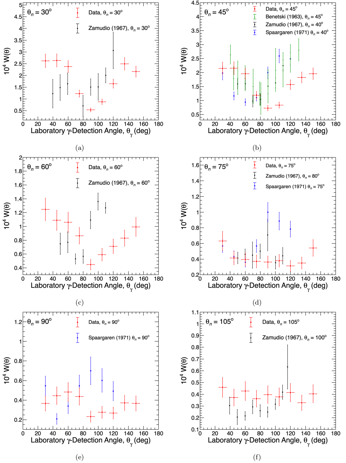
FIG. 12: The results for the normalized correlated n\text{-}\gamma distribution data at E_\alpha \approx 14 MeV are shown here as \gamma distributions compared to the available literature data for \theta_n = 30^\circ in panel (a), \theta_n = 45^\circ in panel (b), \theta_n = 60^\circ in panel (c), \theta_n = 75^\circ in panel (d), \theta_n = 90^\circ in panel (e), and \theta_n = 105^\circ in panel (f). The literature data on these plots are scaled to the present results.
