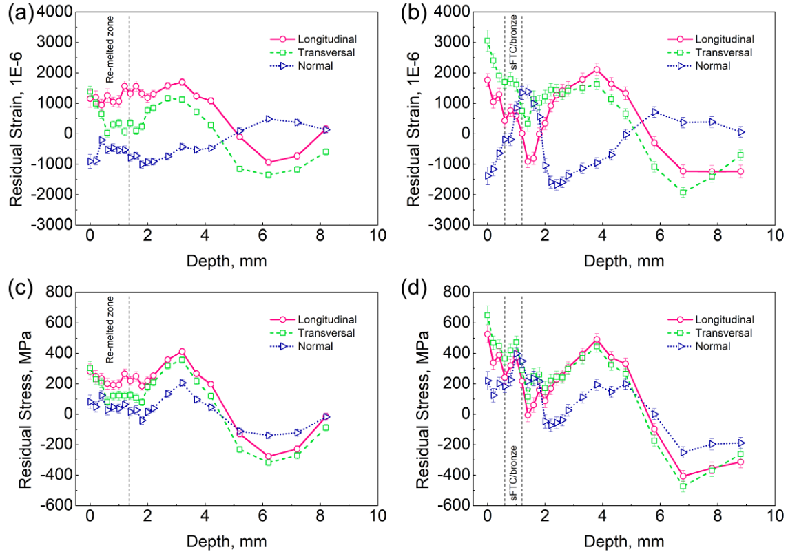
Fig. 6 Neutron diffraction results of the CuAl10Ni5Fe4 bronze-based materials with five laser tracks: residual strains in the Cu matrix of (a) the re-melted bronze and (b) the sFTC/bronze composite deposit; residual stresses in the Cu matrix of (c) the re-melted bronze and (d) the sFTC/bronze composite deposit. The error bars are related to the fitting errors of peak positions.
