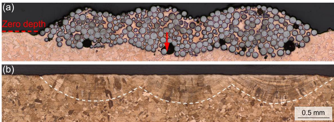
Fig. 2 Microstructures of multi-track laser processed samples: (a) sFTC/Cu composite deposit and (b) re-melted pure Cu. The zero-depth definition for the sFTC/Cu composite deposit is
