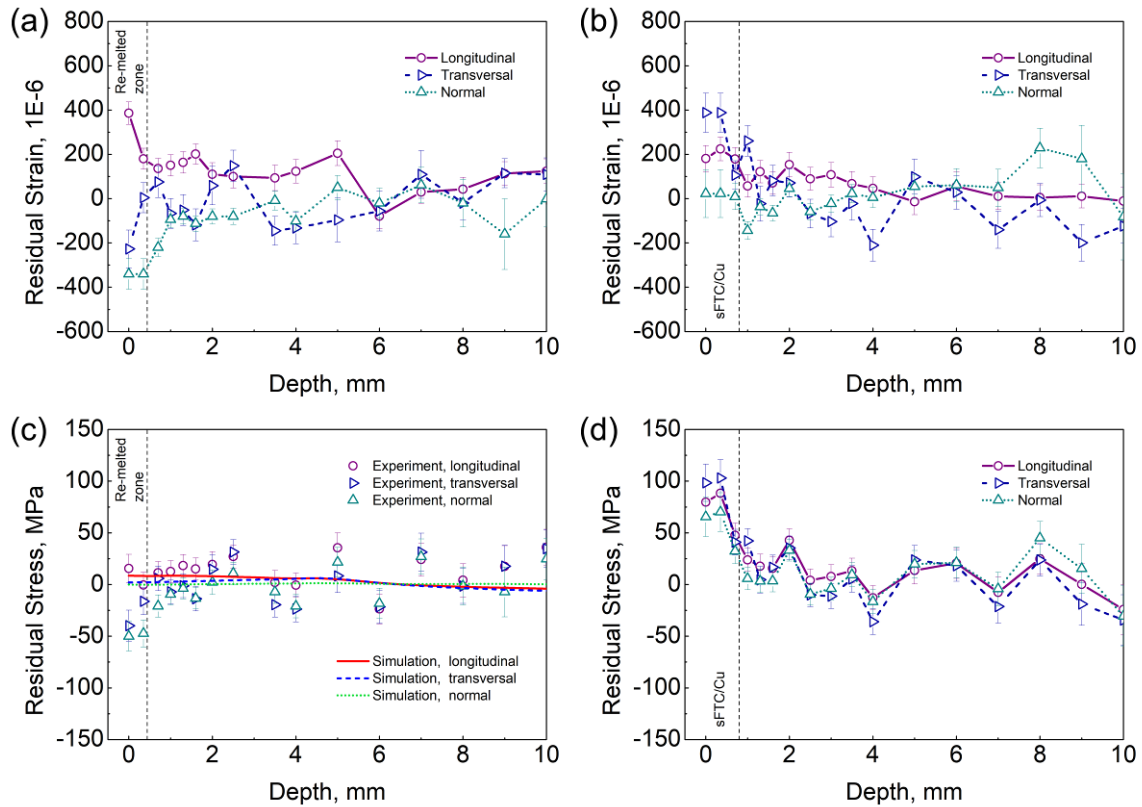
Fig. 4 Neutron diffraction results of the pure Cu-based materials with three laser tracks: residual strains in (a) the re-melted Cu and (b) the Cu matrix of the sFTC/Cu composite deposit; residual stresses in (c) the re-melted Cu and (d) the Cu matrix of the sFTC/Cu composite deposit. The finite element model simulated residual stress results are also shown in (c) for comparison. The error bars are associated with the fitting errors of the peak
