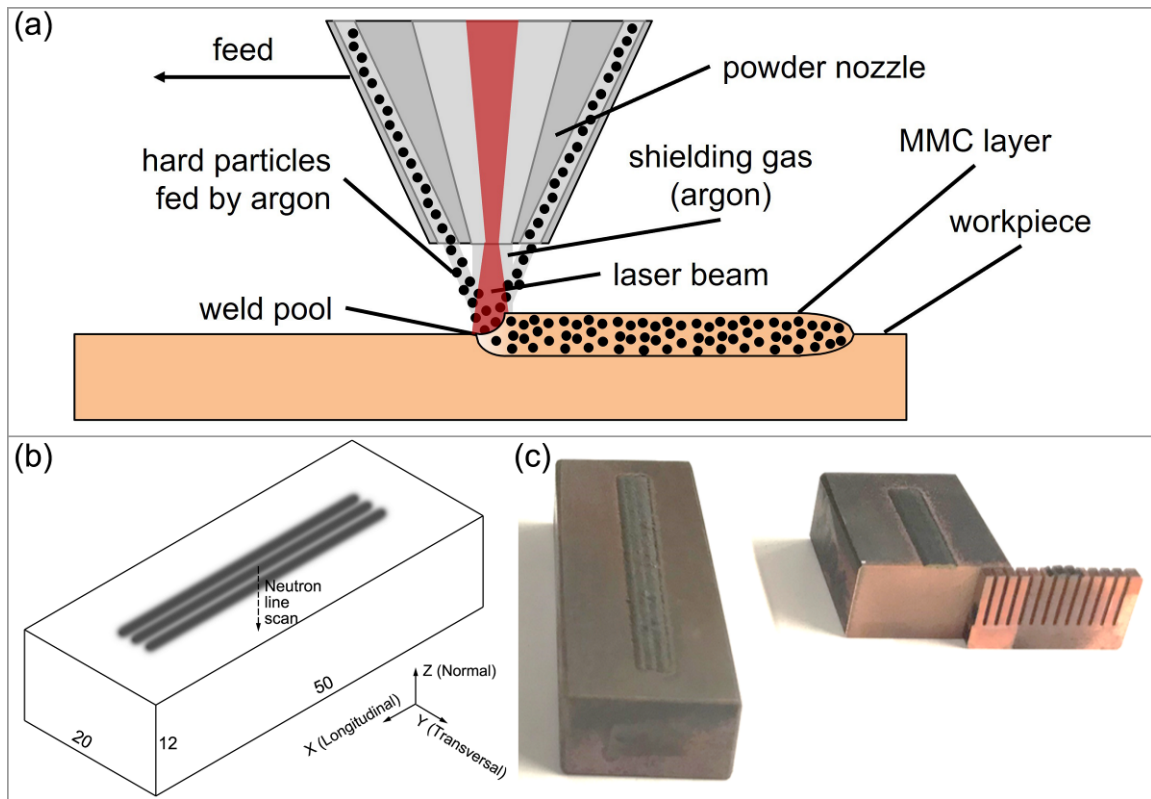
Fig. 1 The samples: (a) a schematic diagram of manufacturing the samples using a laser melt injection process [17]; (b) the coordinate system for the neutron diffraction scan with the origin at the middle of the center laser track; (c) the real sFTC/Cu composite deposit brick and the corresponding comb. Note that the zero-depth positions for the sFTC/Cu and sFTC/bronze composite deposit bricks are defined in Fig. 2(a) and Fig. 3(a), respectively.
