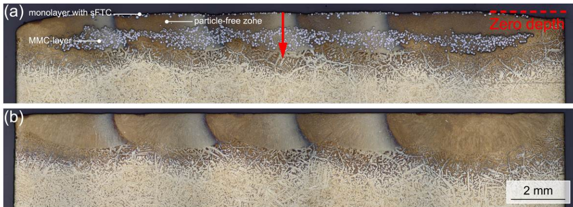
Fig. 3 Microstructures of multi-track laser processed samples: (a) sFTC/bronze composite deposit and (b) re-melted bronze. The zero-depth definition for the sFTC/bronze composite deposit is used in Fig. 6, and the red arrow indicates the neutron scan line and direction.
