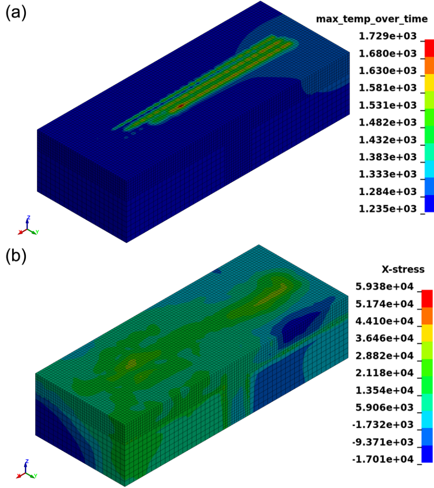
Fig. 5 Predicted (a) maximum temperature ( ^{\circ}\text{C} ) and (b) longitudinal residual stress (Pa) fields.
