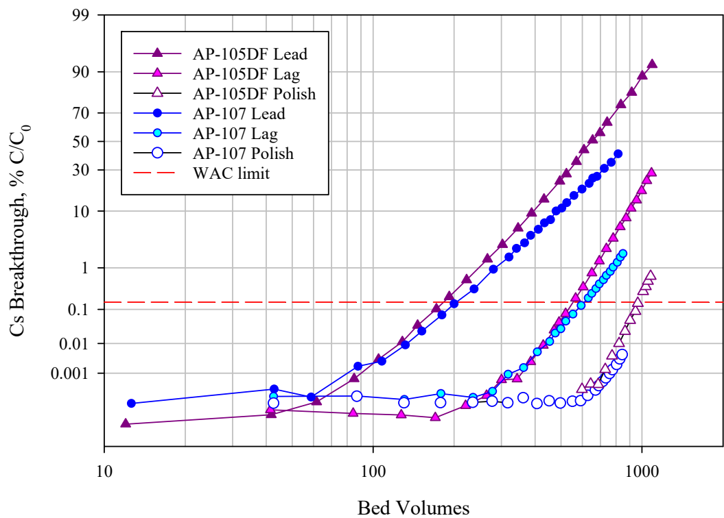
Figure notes: AP-105DF AP-107 Configuration Lead-lag Lead-lag-polish Lead-lag-polish Flowrate, BV/h 1.83 1.88 CST sieve fraction <30 mesh <25 mesh Process Temp. °C 27-29 24-29 Cs, M 5.66E-5 6.91E-5 Na, M 5.92 5.97 K, M 0.102 0.120 OH, M 1.24 0.89 TIC, M 0.472 0.65 Figure 5.6. Load Profile Comparisons: AP-105DF and AP-107 (Fiskum et al. 2019b), CST Lot 2002009604
