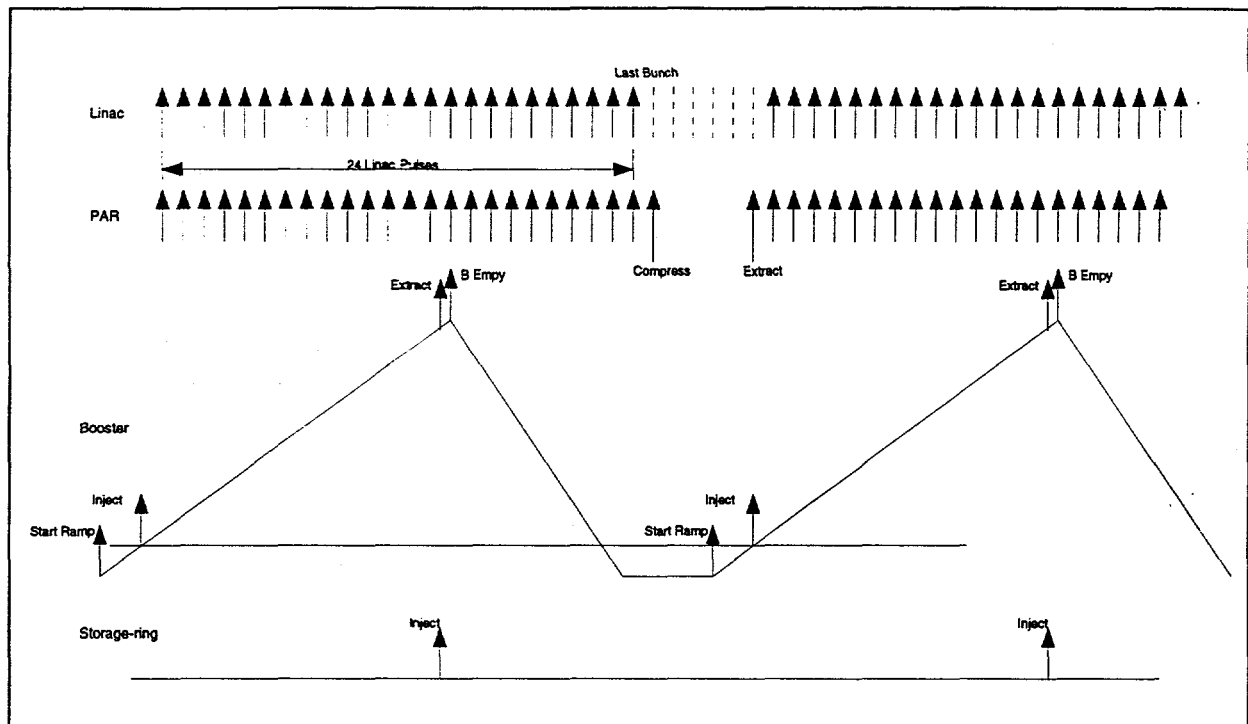
Figure 1 The APS Injection Timing Cycle
