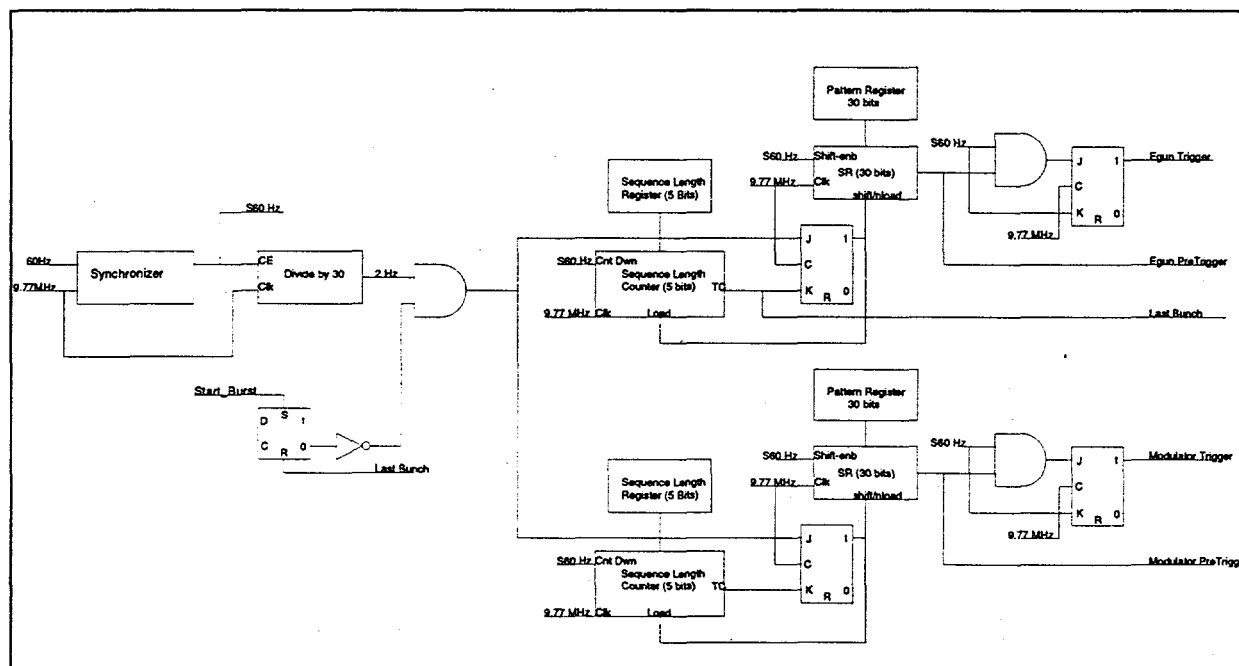
Figure 3 The Linac Injection Sequence Trigger Module Block Diagram
