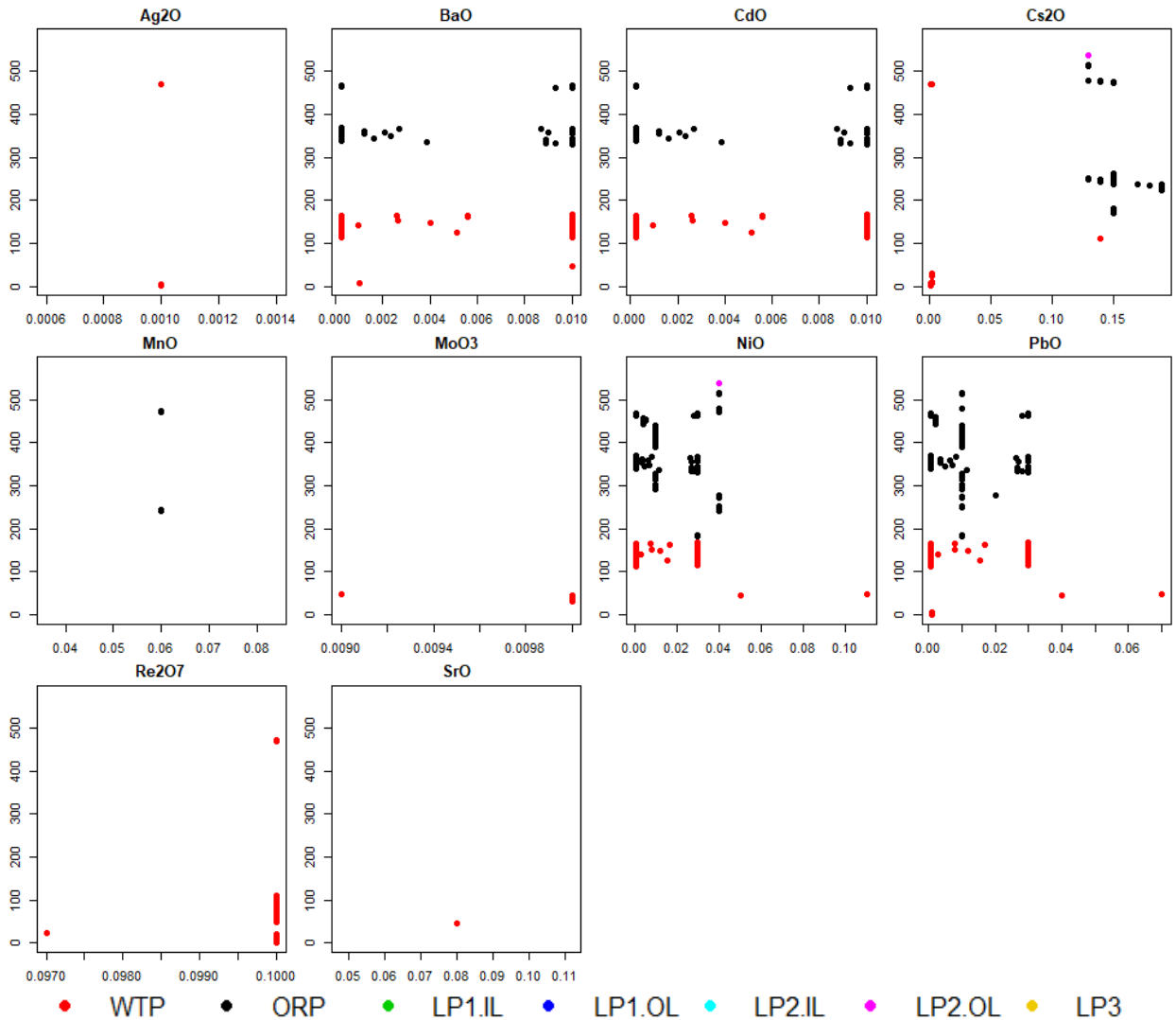
Figure 7.4. Distributions of 10 Minor Components (in mass fractions) for the 576 LAW Glass Compositions with Data for Melter SO 3 Tolerance and Solubility at 1150 °C that Remain after Excluding the 25 Glasses in Table 7.1
