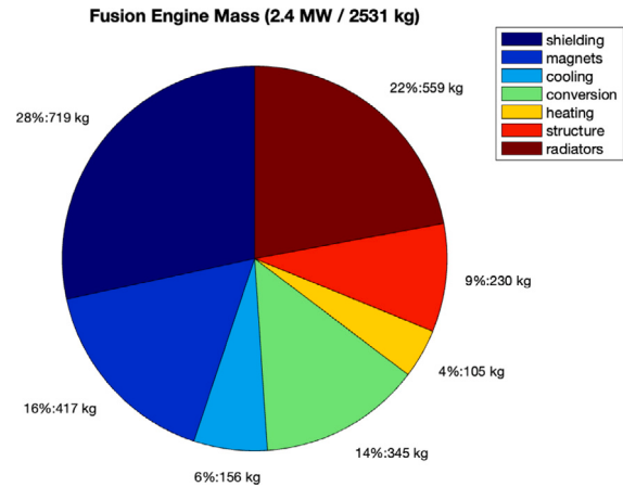
Fig. 10. Mass Breakdown for the transfer vehicle engine.
