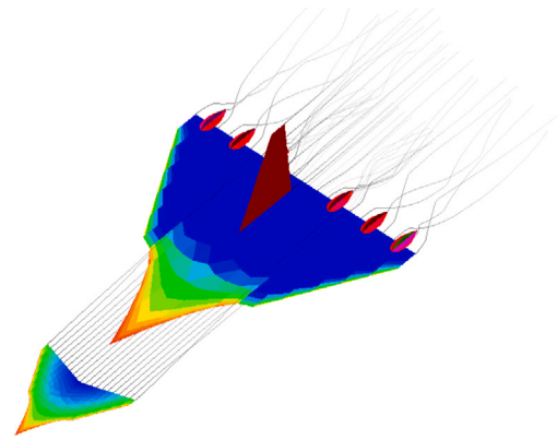
Fig. 24. Trailing Wakes and Vorticity for the Final Design at Angle of Attack of 4.11^\circ .
