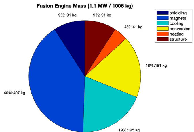
Fig. 12. Mass Breakdown for the aircraft engine.
