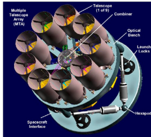
Fig. 5. MIDAS sensor [16].
