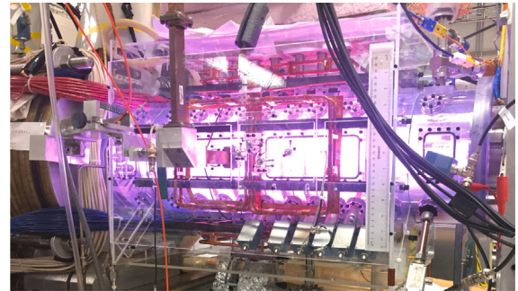
Fig. 6. A plasma shot in the PFRC-2 experiment at PPPL.
