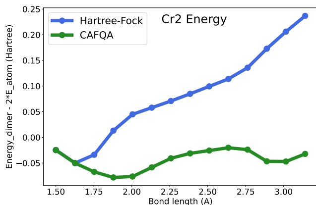
Figure 12: Ground state energy for \text{Cr}_2 with lower 18 out of 36 orbitals frozen. CAFQA’s estimates are limited by computational time / resources, thus Clifford estimates can be suboptimal. Comparison to HF is shown.
