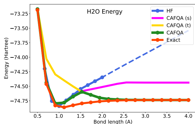
(a) H_2O Energy
