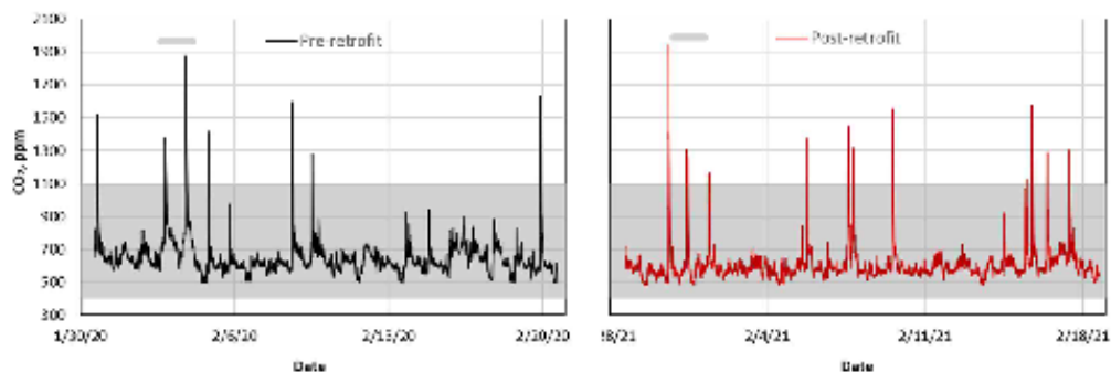
Figure 2. Carbon dioxide levels before and after retrofit
