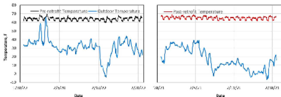
Figure 1. Indoor and outdoor temperatures
