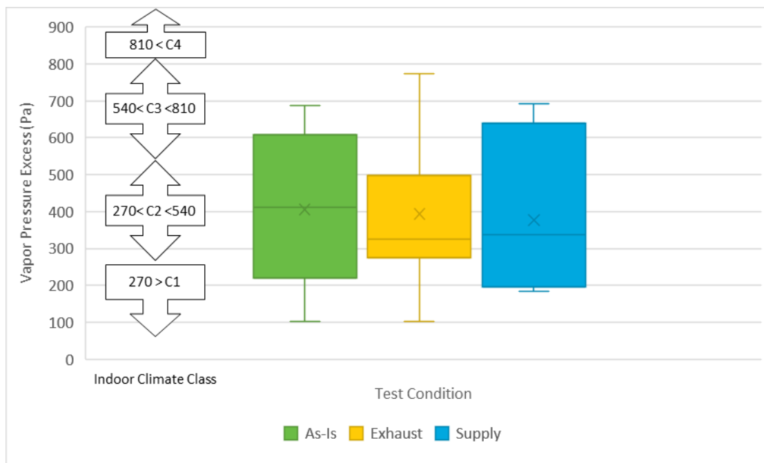
Figure 23. Phase 2 moisture balance readings [n=11]
