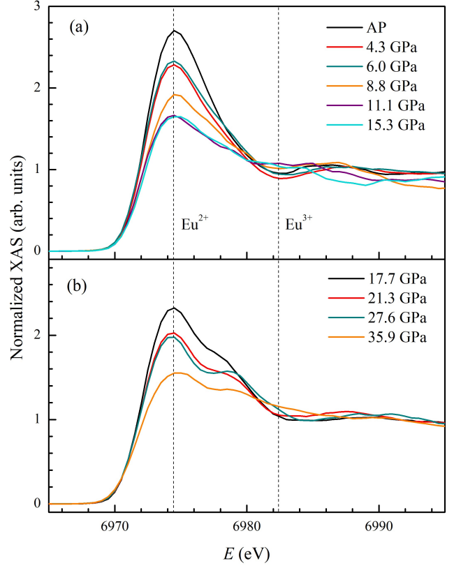
FIG. 5. PFY-XAS plot for \text{Eu } L_3 edge in \text{EuCd}_2\text{As}_2 for different pressures ranging from ambient pressure (AP) to 35.9 GPa taken at room temperature.
