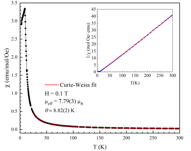
FIG. 8. Magnetic susceptibility data with zero field cooling and Curie-Weiss fitting for the data in 25-300 K region. The plot of 1/\chi is shown in the inset.
