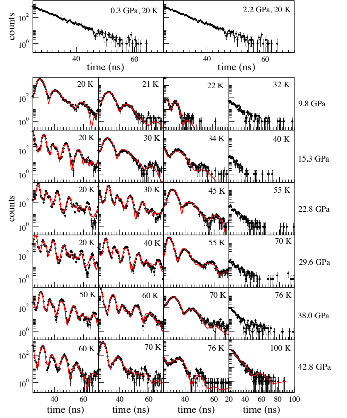
FIG. 1. SMS spectra of ^{151}\text{Eu} in \text{EuCd}_2\text{As}_2 . The black dots represent the experimental data and red lines correspond to fits from CONUSS program.
