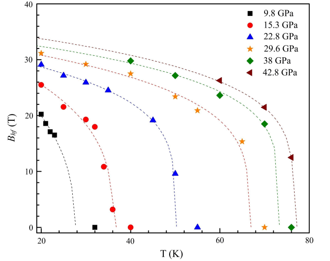
FIG. 2. Extracted magnetic hyperfine field of ^{151}\text{Eu} in \text{EuCd}_2\text{As}_2 as a function of temperature at various pressures. The dashed lines serve as a guide to the eye.
