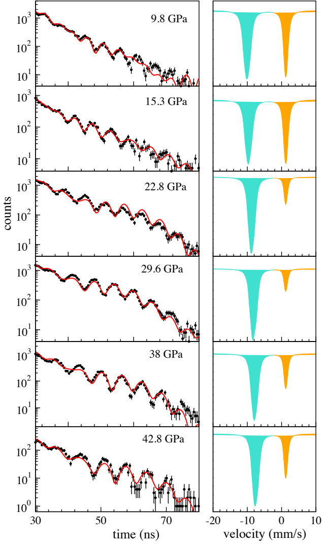
FIG. 4. ^{151}\text{Eu} SMS spectra for various pressures at 100K in \text{EuCd}_2\text{As}_2 with \text{Eu}_2\text{O}_3 as reference which is located at ambient conditions. The simulated energy-domain spectra corresponding to each pressure are plotted in the right column with shaded blue lines representing resonant absorption from \text{EuCd}_2\text{As}_2 and shaded orange lines representing absorption from reference sample \text{Eu}_2\text{O}_3 .
